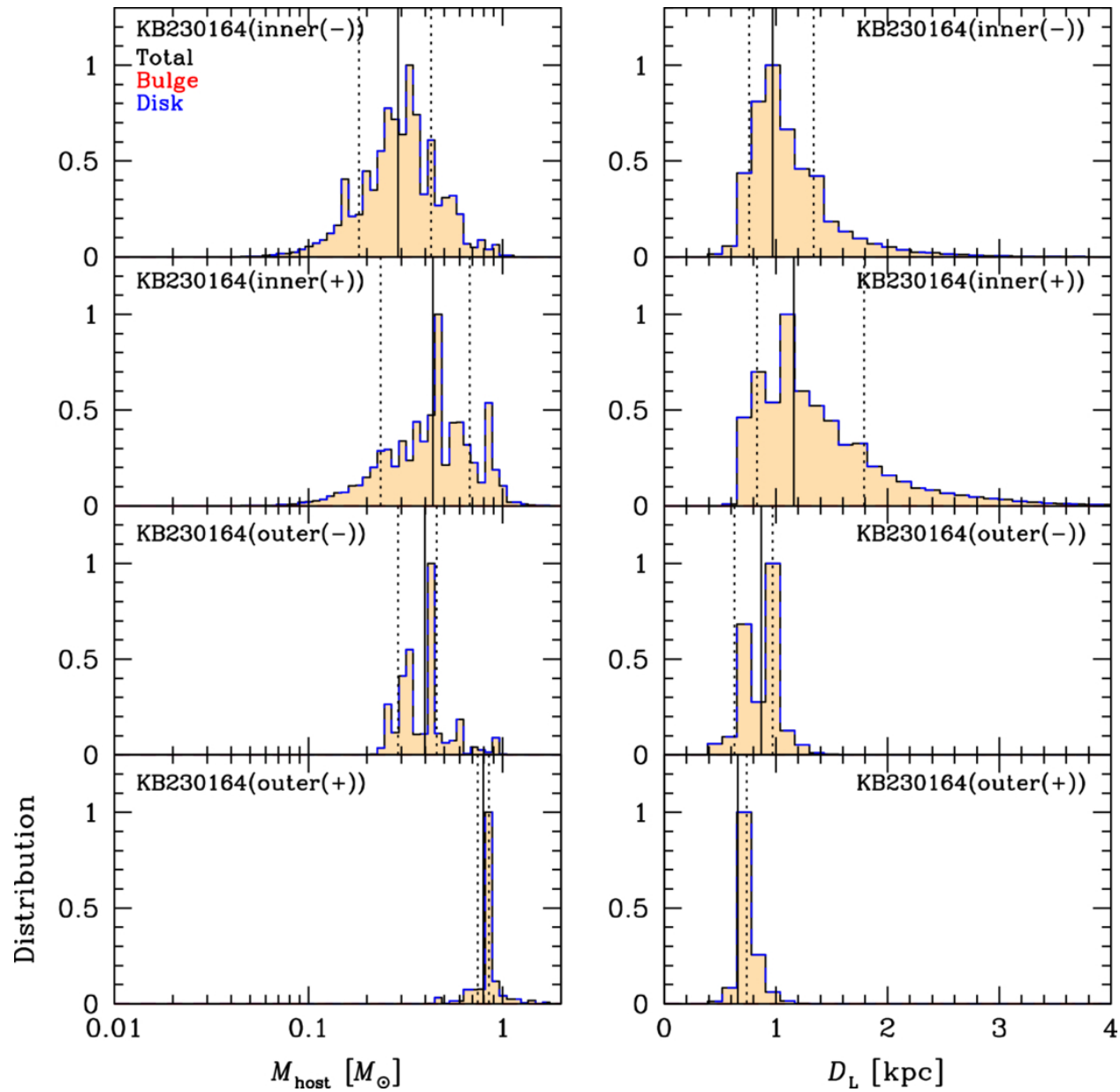
Figure 7. from Yoon-Hyun Ryu et al 2026 Astron. J. 171 doi:10.3847/1538-3881/ae4edf https://dx.doi.org/10.3847/1538-3881/ae4edf © 2026. The Author(s). Published by the American Astronomical Society.
