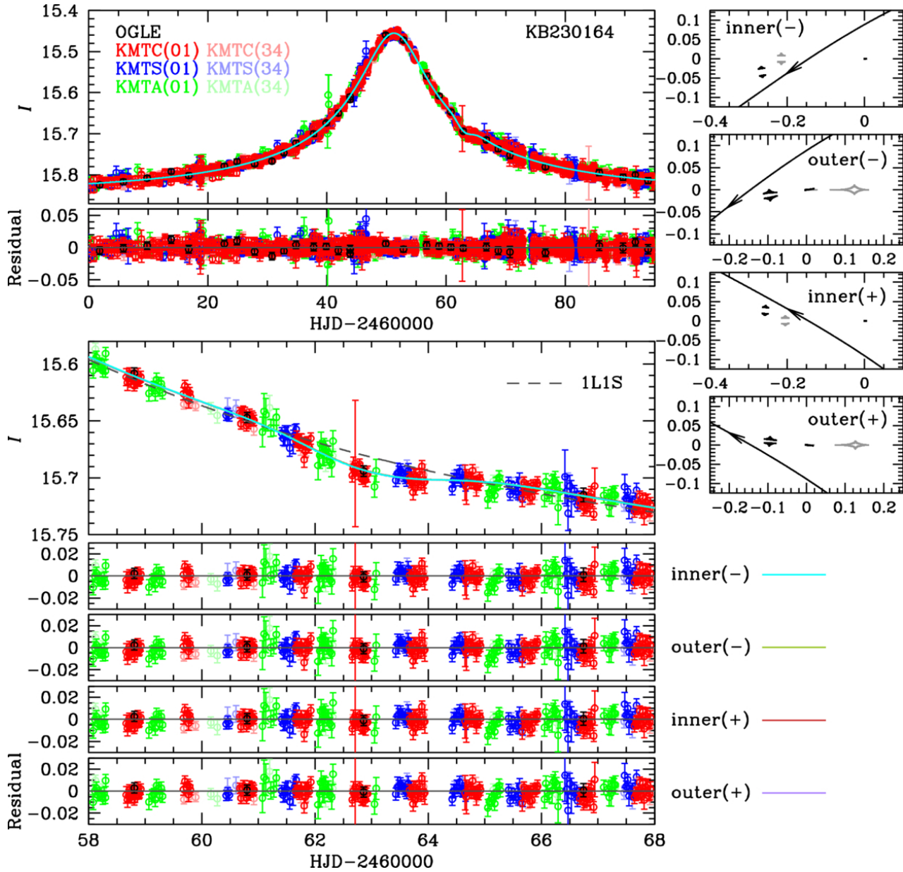
Figure 3. from Yoon-Hyun Ryu et al 2026 Astron. J. 171 doi:10.3847/1538-3881/ae4edf https://dx.doi.org/10.3847/1538-3881/ae4edf © 2026. The Author(s). Published by the American Astronomical Society.
