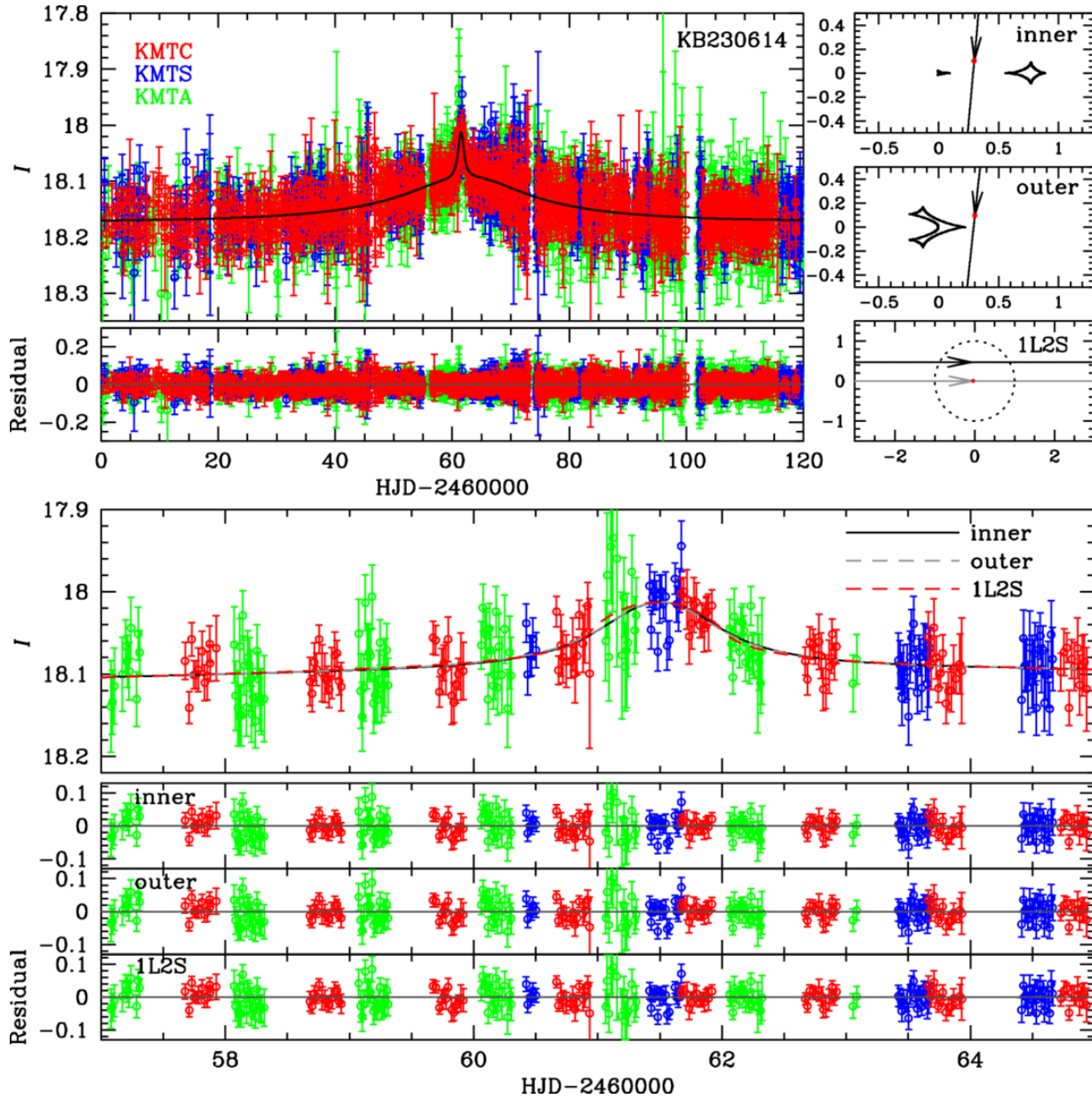
Figure 18. from Yoon-Hyun Ryu et al 2026 Astron. J. 171 doi:10.3847/1538-3881/ae4edf https://dx.doi.org/10.3847/1538-3881/ae4edf © 2026. The Author(s). Published by the American Astronomical Society.
