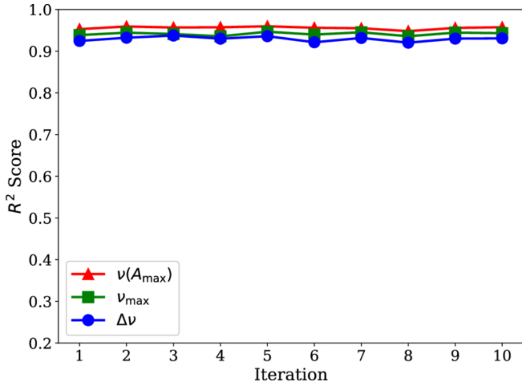
Figure 6. from Akram Bolouki et al 2026 Astron. J. 171 doi:10.3847/1538-3881/ae4bd8 https://dx.doi.org/10.3847/1538-3881/ae4bd8 © 2026. The Author(s). Published by the American Astronomical Society.
