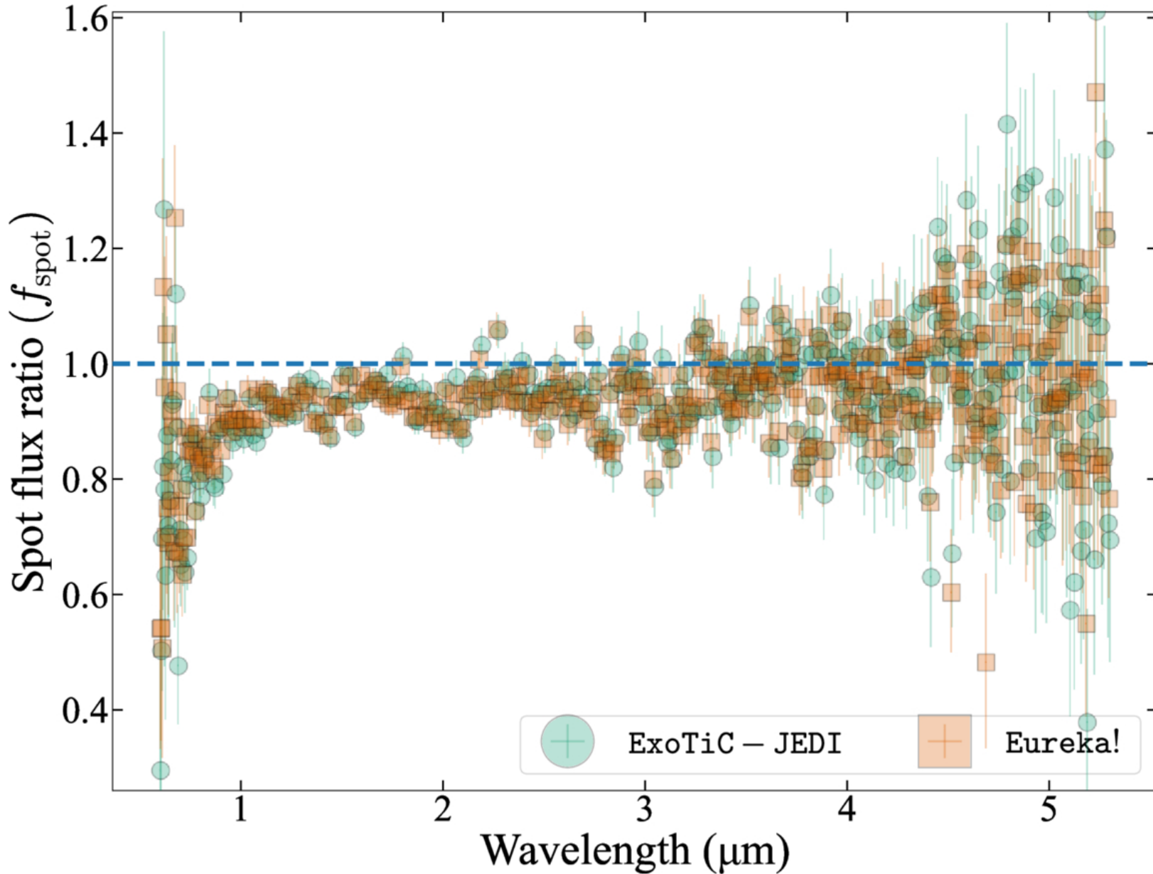
Figure 15. Spot contrasts from the spectroscopic fits. from Caleb I. Cañas et al 2026 Astron. J. 171 doi:10.3847/1538-3881/ae4976 https://dx.doi.org/10.3847/1538-3881/ae4976 © 2026. The Author(s). Published by the American Astronomical Society.
