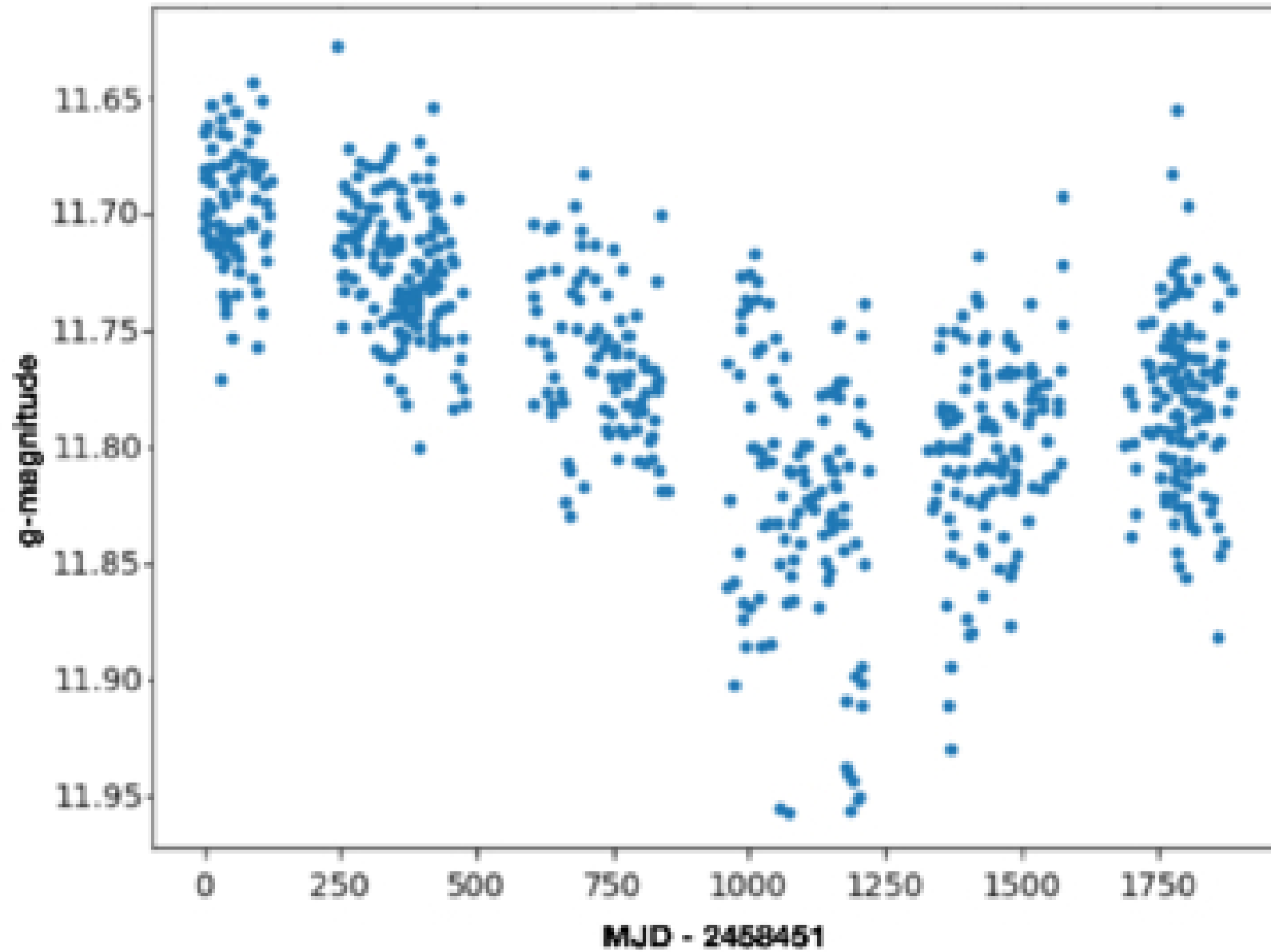
Figure 7. from Bo Reipurth et al 2026 Astron. J. 171 doi:10.3847/1538-3881/ae4962 https://dx.doi.org/10.3847/1538-3881/ae4962 © 2026. The Author(s). Published by the American Astronomical Society.
