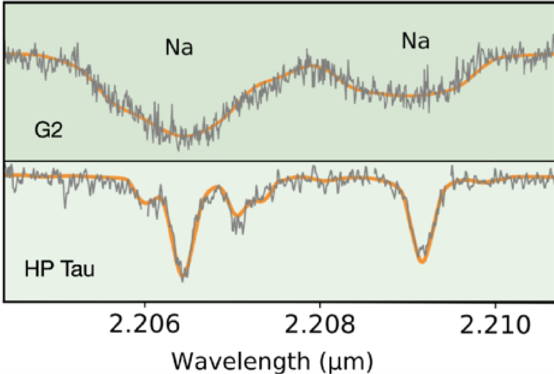
Figure 6. from Bo Reipurth et al 2026 Astron. J. 171 doi:10.3847/1538-3881/ae4962 https://dx.doi.org/10.3847/1538-3881/ae4962 © 2026. The Author(s). Published by the American Astronomical Society.
