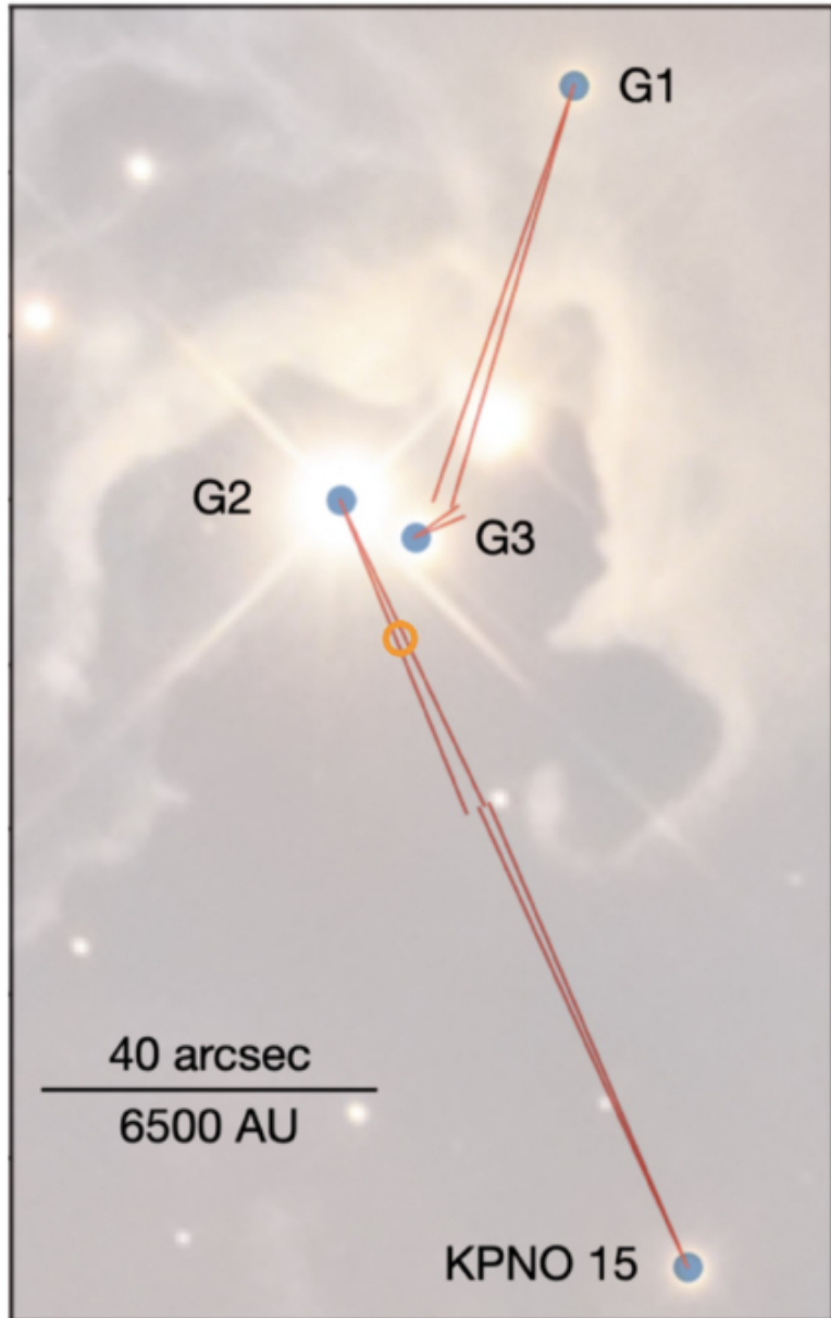
Figure 3. from Bo Reipurth et al 2026 Astron. J. 171 doi:10.3847/1538-3881/ae4962 https://dx.doi.org/10.3847/1538-3881/ae4962 © 2026. The Author(s). Published by the American Astronomical Society.
