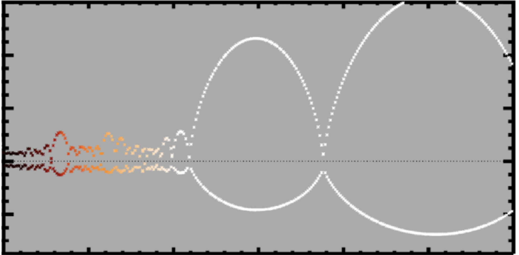
Figure 14. from Bo Reipurth et al 2026 Astron. J. 171 doi:10.3847/1538-3881/ae4962 https://dx.doi.org/10.3847/1538-3881/ae4962 © 2026. The Author(s). Published by the American Astronomical Society.
