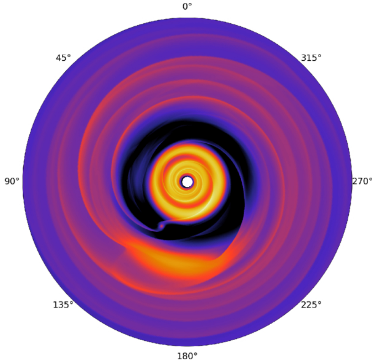
Figure 10. from Janus Kozdon et al 2026 Astron. J. 171 doi:10.3847/1538-3881/ae48f6 https://dx.doi.org/10.3847/1538-3881/ae48f6 © 2026. The Author(s). Published by the American Astronomical Society.
