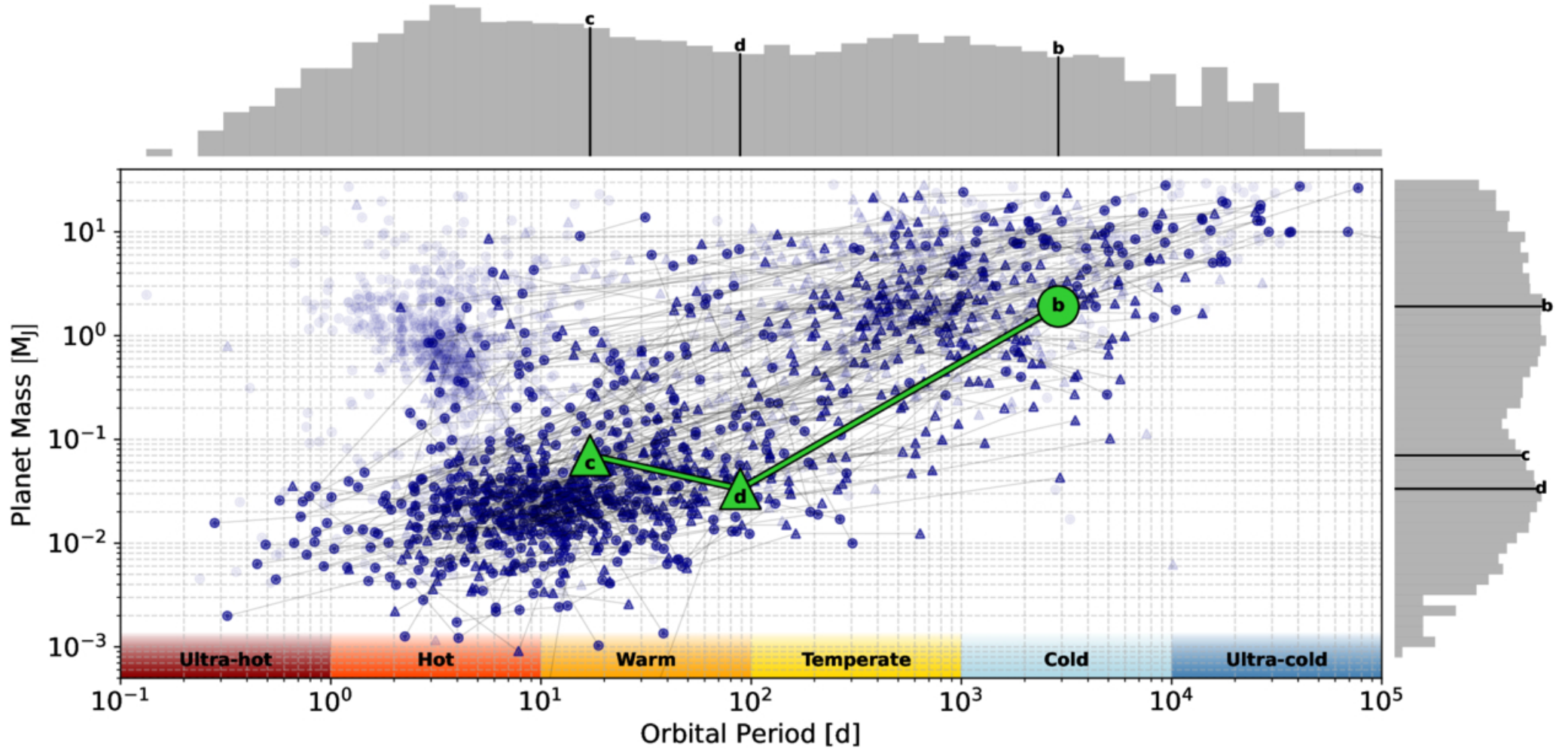
Figure 7. from Mark R. Giovinazzi et al 2026 Astron. J. 171 doi:10.3847/1538-3881/ae48f1 https://dx.doi.org/10.3847/1538-3881/ae48f1 © 2026. The Author(s). Published by the American Astronomical Society.
