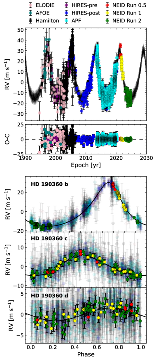
Figure 2. from Mark R. Giovinazzi et al 2026 Astron. J. 171 doi:10.3847/1538-3881/ae48f1 https://dx.doi.org/10.3847/1538-3881/ae48f1 © 2026. The Author(s). Published by the American Astronomical Society.
