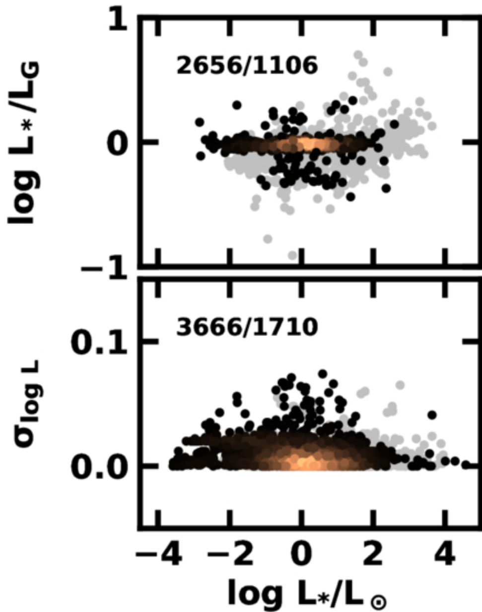
Figure 9. from Scott J. Kenyon et al 2026 Astron. J. 171 doi:10.3847/1538-3881/ae46a2 https://dx.doi.org/10.3847/1538-3881/ae46a2 © 2026. The Author(s). Published by the American Astronomical Society.
