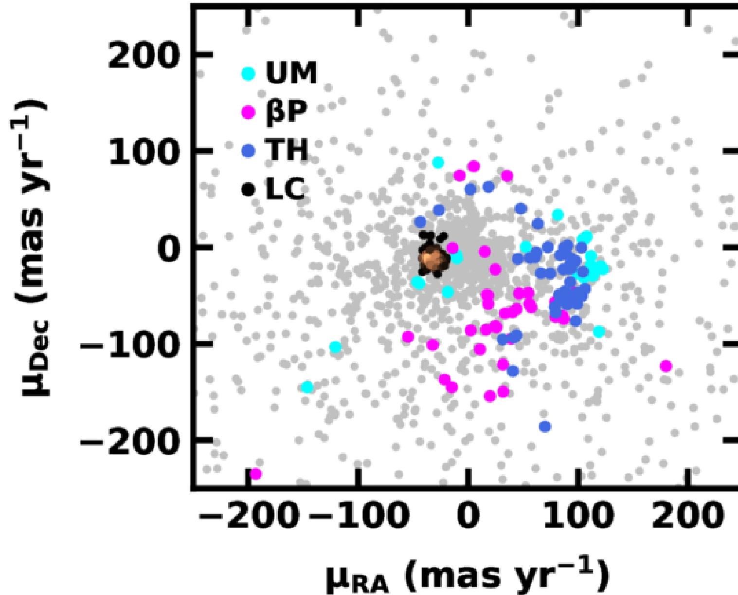
Figure 19. from Scott J. Kenyon et al 2026 Astron. J. 171 doi:10.3847/1538-3881/ae46a2 https://dx.doi.org/10.3847/1538-3881/ae46a2 © 2026. The Author(s). Published by the American Astronomical Society.
