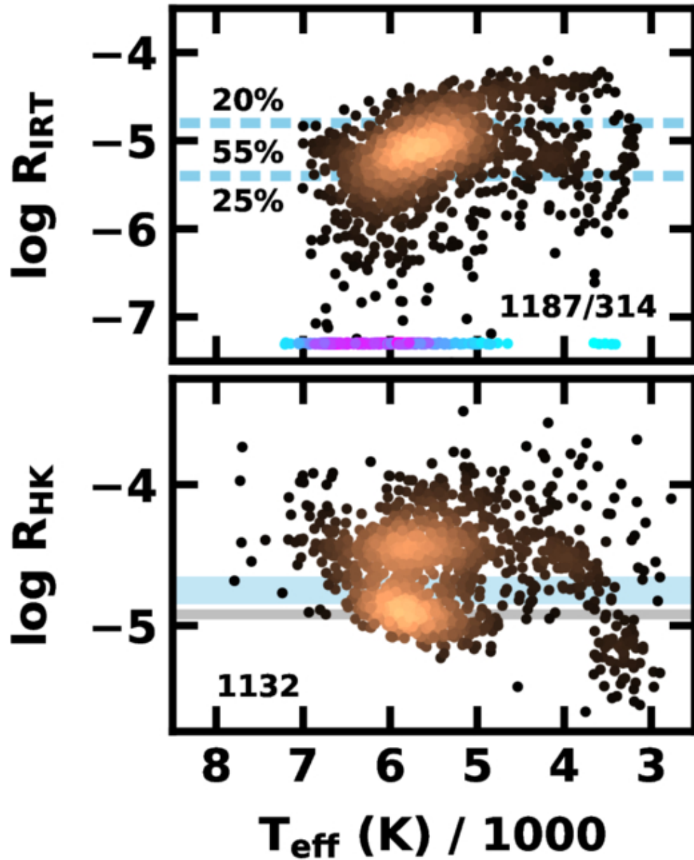
Figure 14. from Scott J. Kenyon et al 2026 Astron. J. 171 doi:10.3847/1538-3881/ae46a2 https://dx.doi.org/10.3847/1538-3881/ae46a2 © 2026. The Author(s). Published by the American Astronomical Society.
