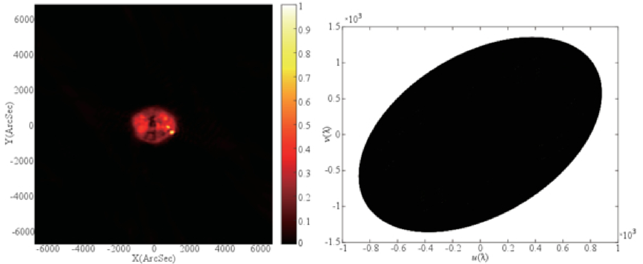
Figure 9. from Xiaocheng Yang et al 2026 Astron. J. 171 doi:10.3847/1538-3881/ae45a1 https://dx.doi.org/10.3847/1538-3881/ae45a1 © 2026. The Author(s). Published by the American Astronomical Society.
