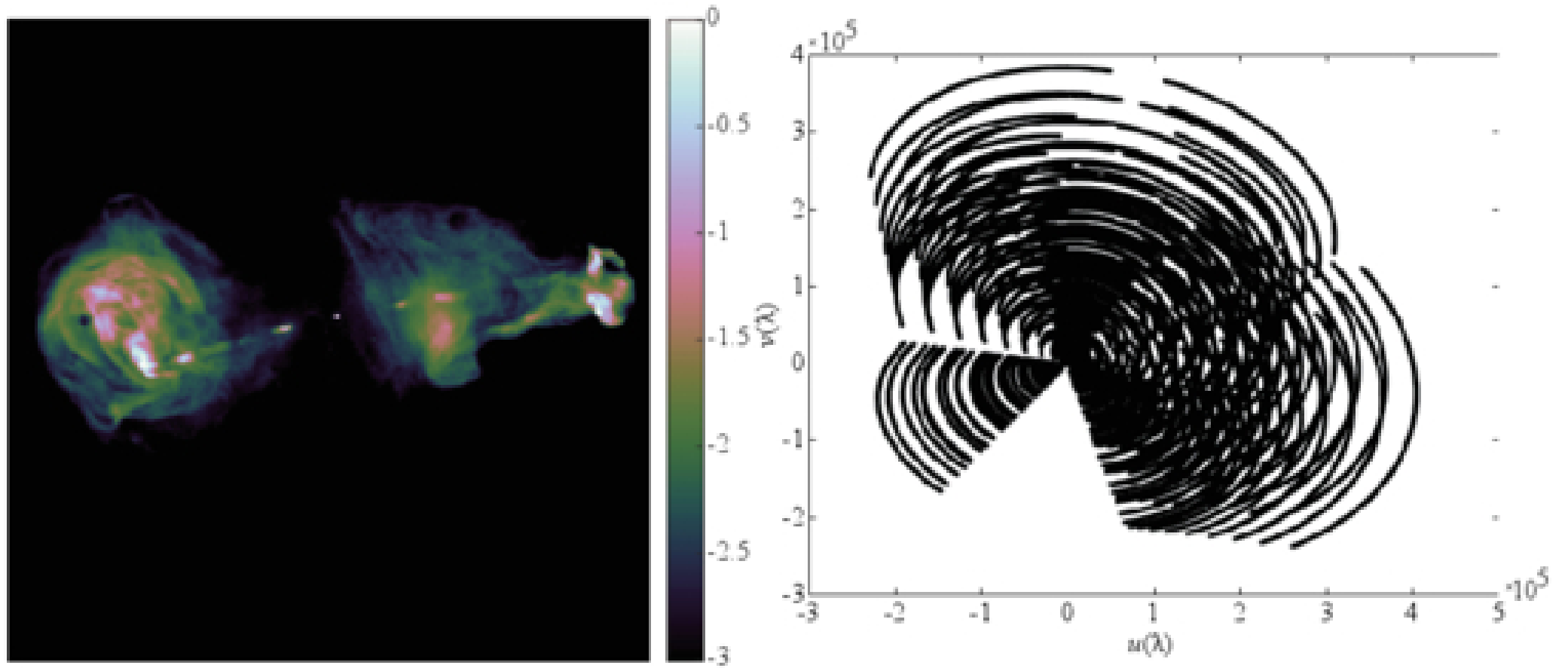
Figure 2. from Xiaocheng Yang et al 2026 Astron. J. 171 doi:10.3847/1538-3881/ae45a1 https://dx.doi.org/10.3847/1538-3881/ae45a1 © 2026. The Author(s). Published by the American Astronomical Society.
