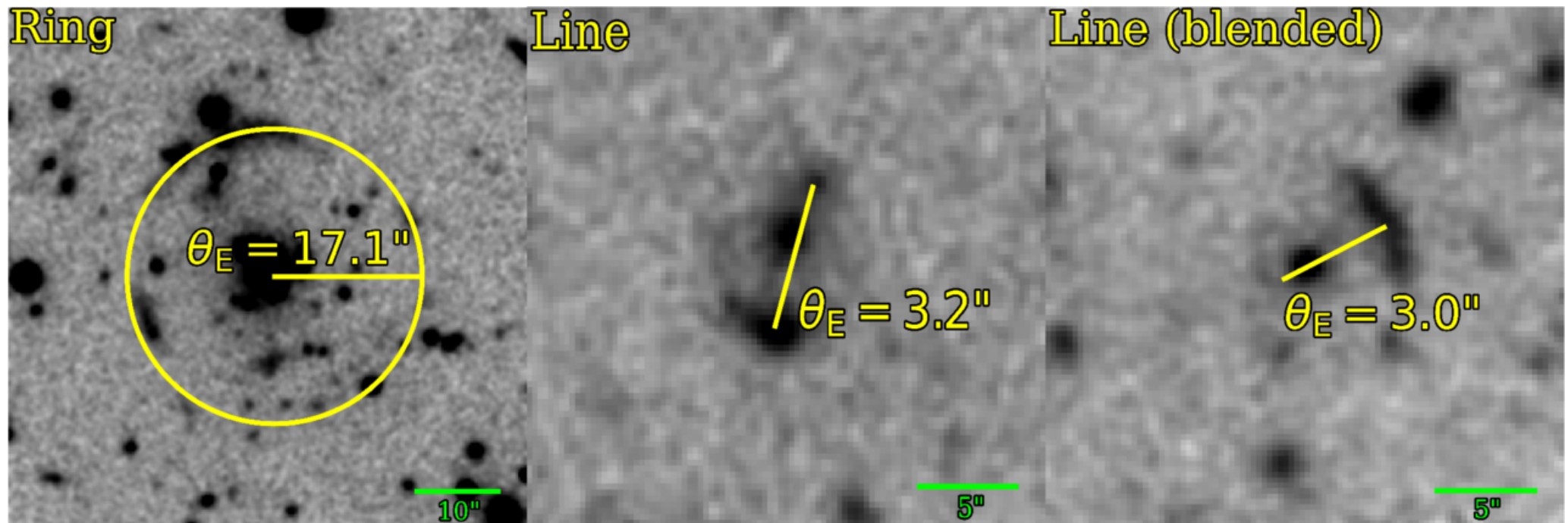
Figure 6. from William J. Gottemoller et al 2026 Astron. J. 171 doi:10.3847/1538-3881/ae4480 https://dx.doi.org/10.3847/1538-3881/ae4480 © 2026. The Author(s). Published by the American Astronomical Society.
