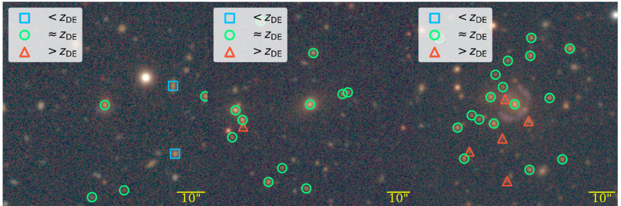
Figure 4. from William J. Gottemoller et al 2026 Astron. J. 171 doi:10.3847/1538-3881/ae4480 https://dx.doi.org/10.3847/1538-3881/ae4480 © 2026. The Author(s). Published by the American Astronomical Society.
