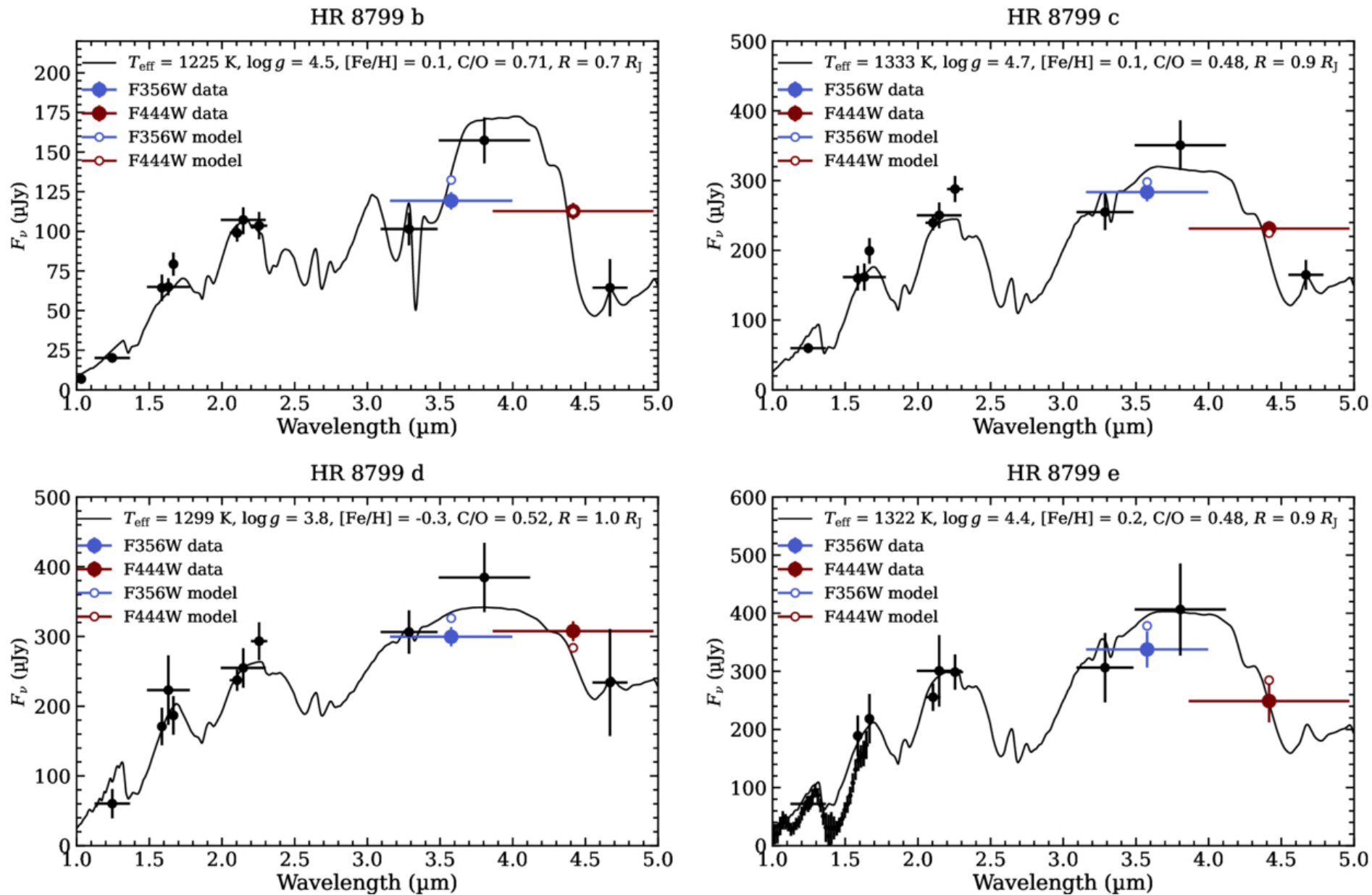
Figure 7. from Bryden Geoffrey et al 2026 Astron. J. 171 doi:10.3847/1538-3881/ae43e8 https://dx.doi.org/10.3847/1538-3881/ae43e8 © 2026. The Author(s). Published by the American Astronomical Society.
