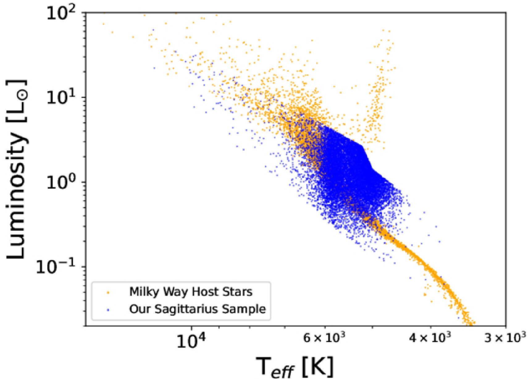
Figure 4. from William Schap et al 2026 Astron. J. 171 doi:10.3847/1538-3881/ae4345 https://dx.doi.org/10.3847/1538-3881/ae4345 © 2026. The Author(s). Published by the American Astronomical Society.
