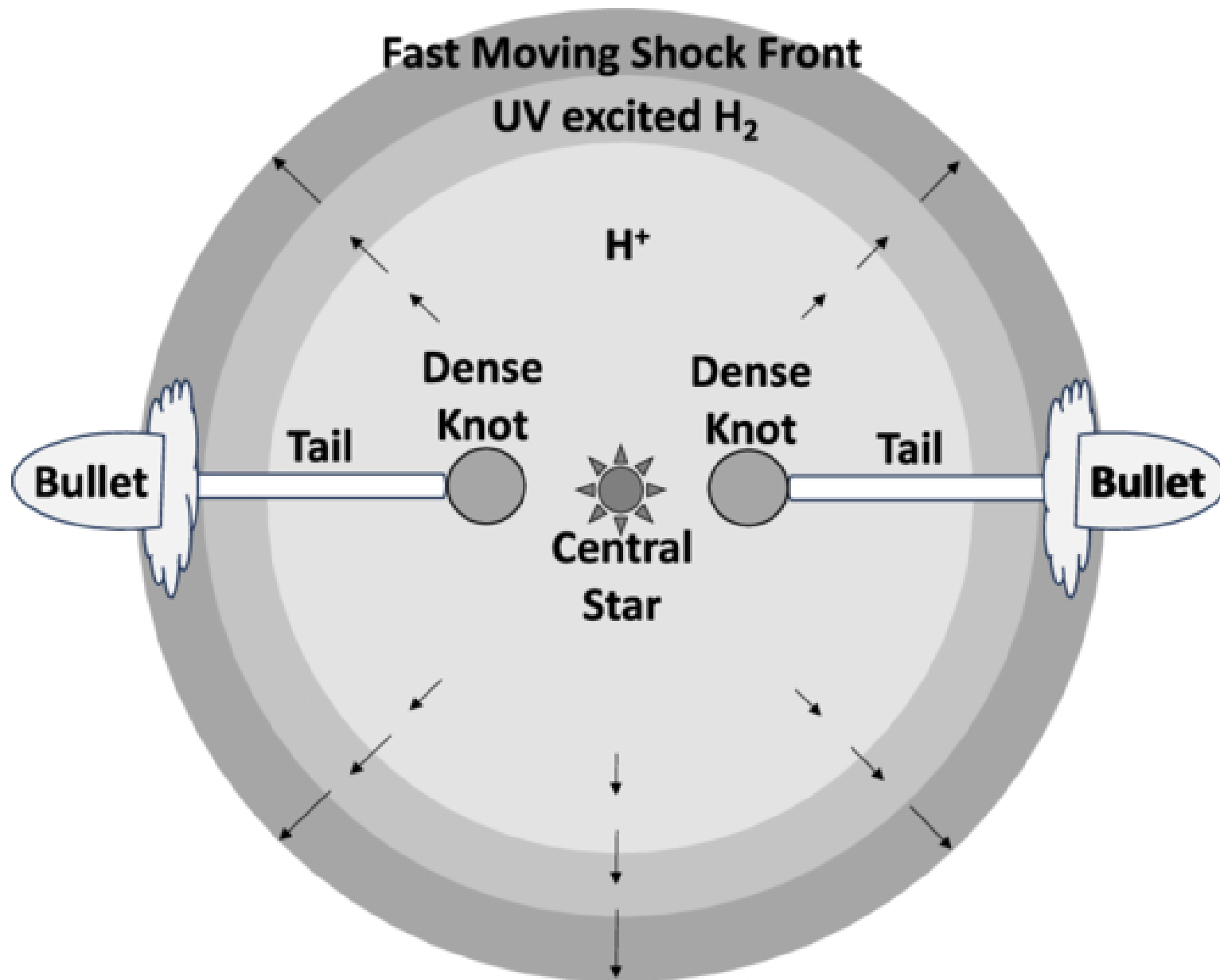
Figure 10. from Kyle F. Kaplan et al 2026 Astron. J. 171 doi:10.3847/1538-3881/ae40ac https://dx.doi.org/10.3847/1538-3881/ae40ac © 2026. The Author(s). Published by the American Astronomical Society.
