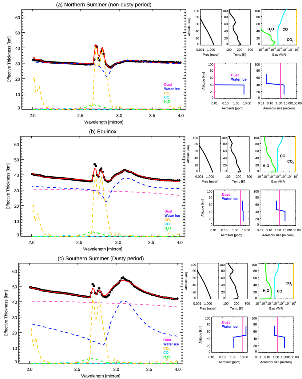
Figure 6. from Shohei Aoki et al 2026 Astron. J. 171 doi:10.3847/1538-3881/ae3da7 https://dx.doi.org/10.3847/1538-3881/ae3da7 © 2026. The Author(s). Published by the American Astronomical Society.
