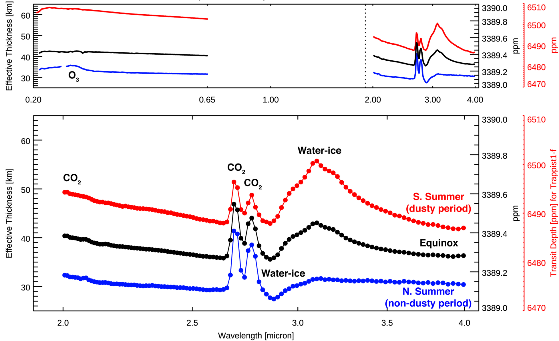
Figure 5. from Shohei Aoki et al 2026 Astron. J. 171 doi:10.3847/1538-3881/ae3da7 https://dx.doi.org/10.3847/1538-3881/ae3da7 © 2026. The Author(s). Published by the American Astronomical Society.
