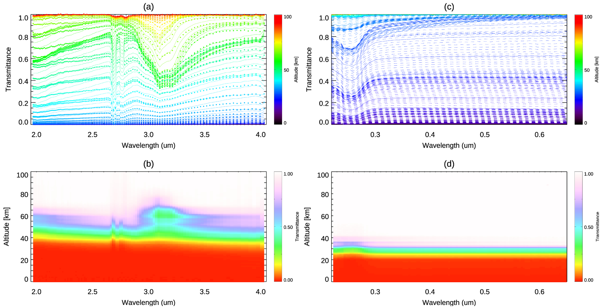
Figure 2. from Shohei Aoki et al 2026 Astron. J. 171 doi:10.3847/1538-3881/ae3da7 https://dx.doi.org/10.3847/1538-3881/ae3da7 © 2026. The Author(s). Published by the American Astronomical Society.
