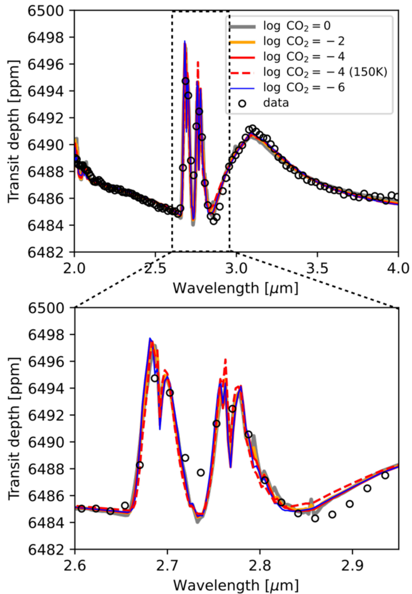
Figure 10. from Shohei Aoki et al 2026 Astron. J. 171 doi:10.3847/1538-3881/ae3da7 https://dx.doi.org/10.3847/1538-3881/ae3da7 © 2026. The Author(s). Published by the American Astronomical Society.
