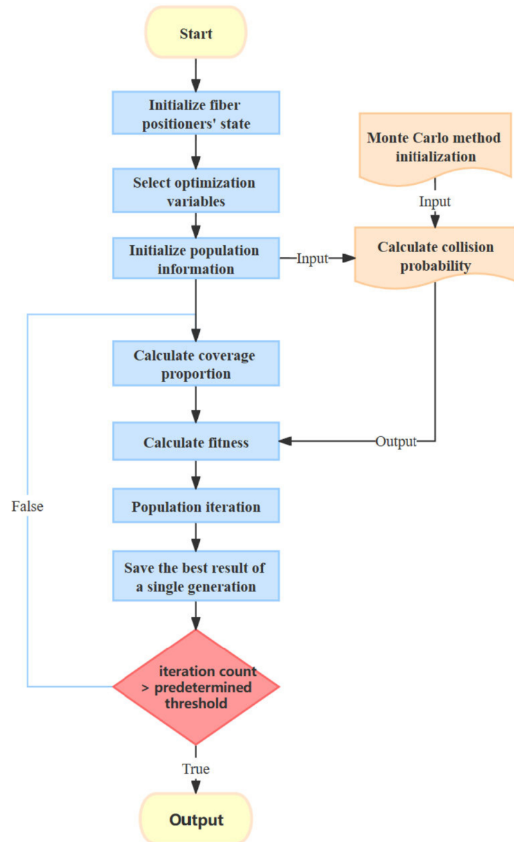
Figure 9. from Zengxiang Zhou et al 2026 Astron. J. 171 doi:10.3847/1538-3881/ae3c82 https://dx.doi.org/10.3847/1538-3881/ae3c82 © 2026. The Author(s). Published by the American Astronomical Society.
