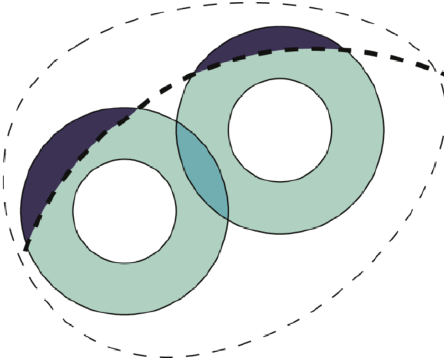
Figure 6. from Zengxiang Zhou et al 2026 Astron. J. 171 doi:10.3847/1538-3881/ae3c82 https://dx.doi.org/10.3847/1538-3881/ae3c82 © 2026. The Author(s). Published by the American Astronomical Society.
