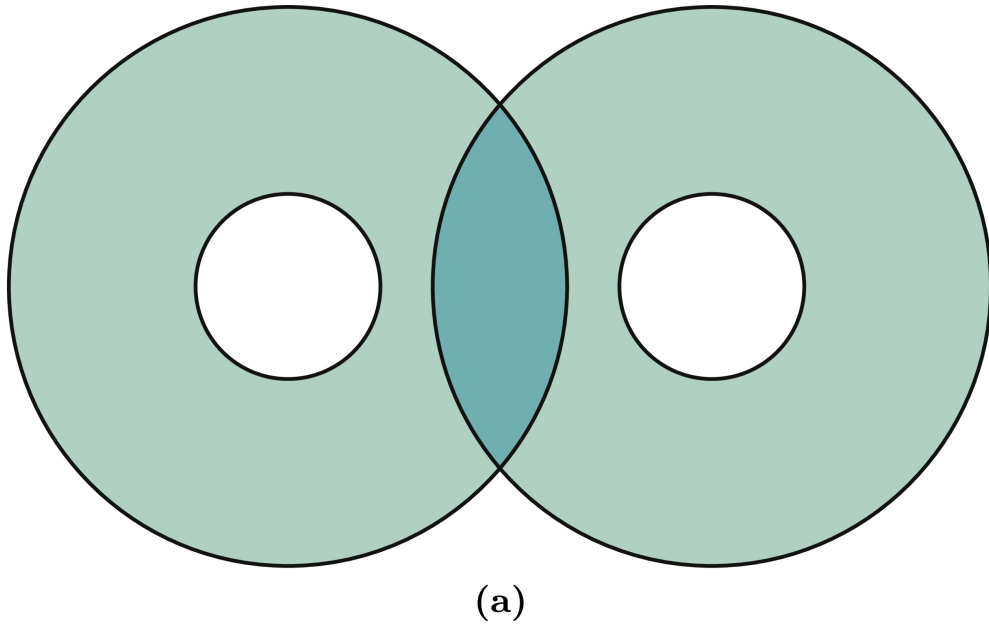
Figure 5. from Zengxiang Zhou et al 2026 Astron. J. 171 doi:10.3847/1538-3881/ae3c82 https://dx.doi.org/10.3847/1538-3881/ae3c82 © 2026. The Author(s). Published by the American Astronomical Society.
