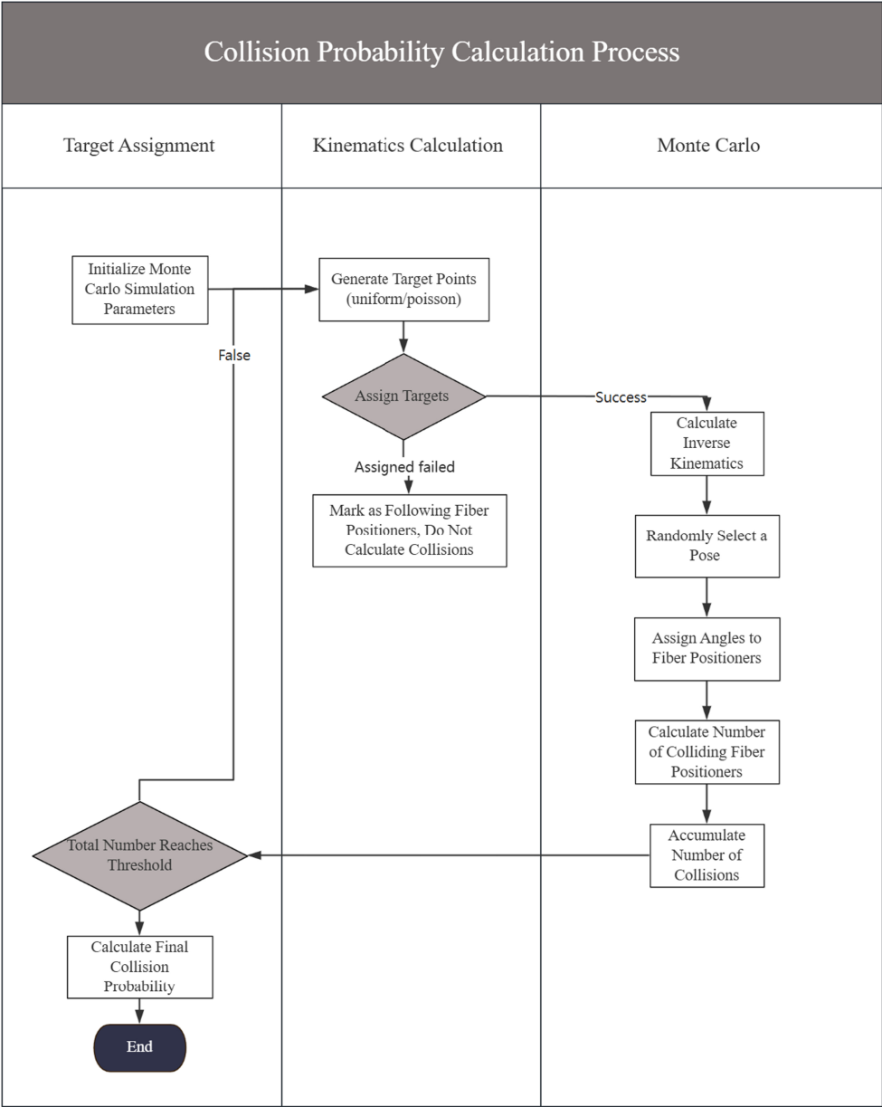
Figure 3. from Zengxiang Zhou et al 2026 Astron. J. 171 doi:10.3847/1538-3881/ae3c82 https://dx.doi.org/10.3847/1538-3881/ae3c82 © 2026. The Author(s). Published by the American Astronomical Society.
