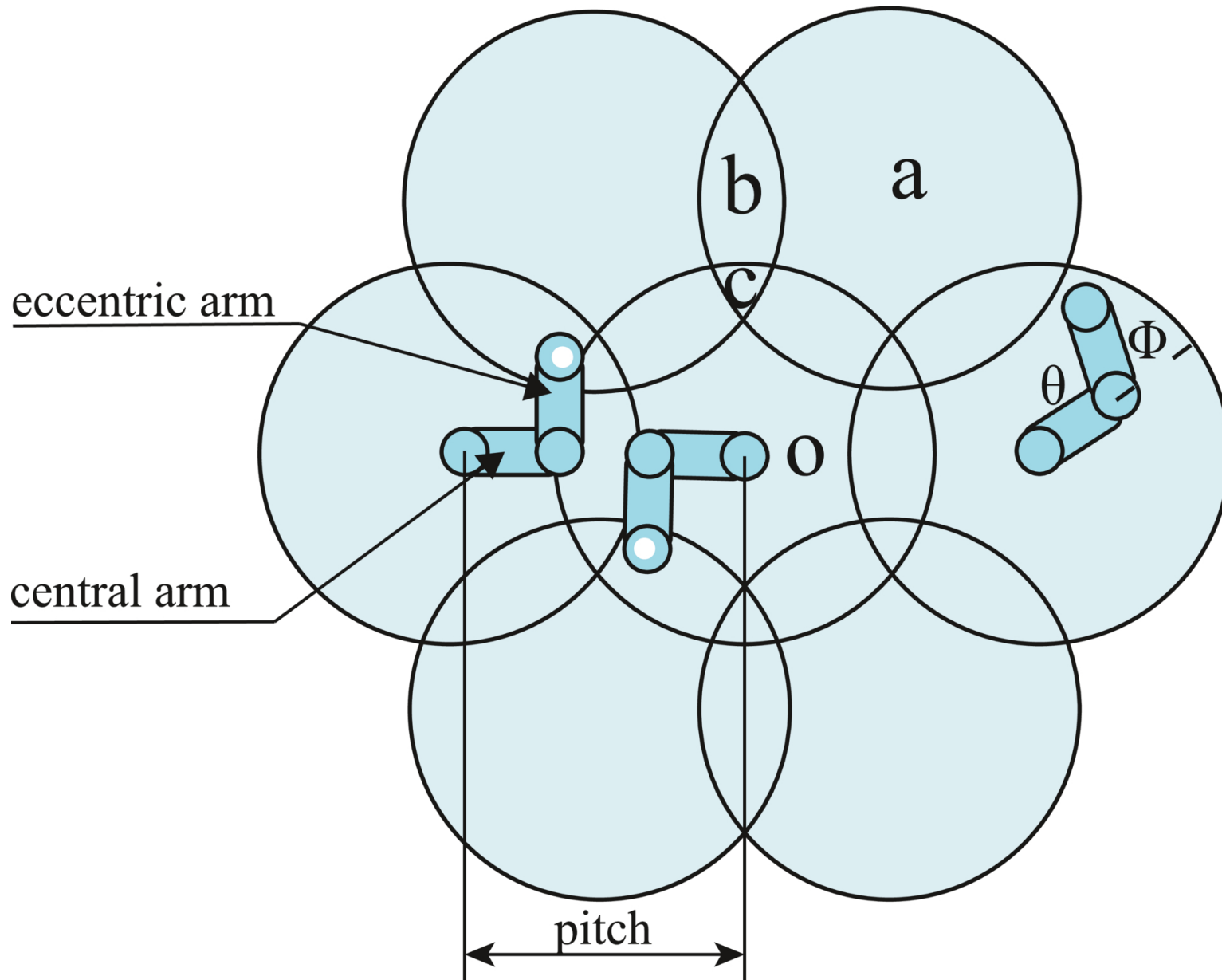
Figure 2. from Zengxiang Zhou et al 2026 Astron. J. 171 doi:10.3847/1538-3881/ae3c82 https://dx.doi.org/10.3847/1538-3881/ae3c82 © 2026. The Author(s). Published by the American Astronomical Society.
