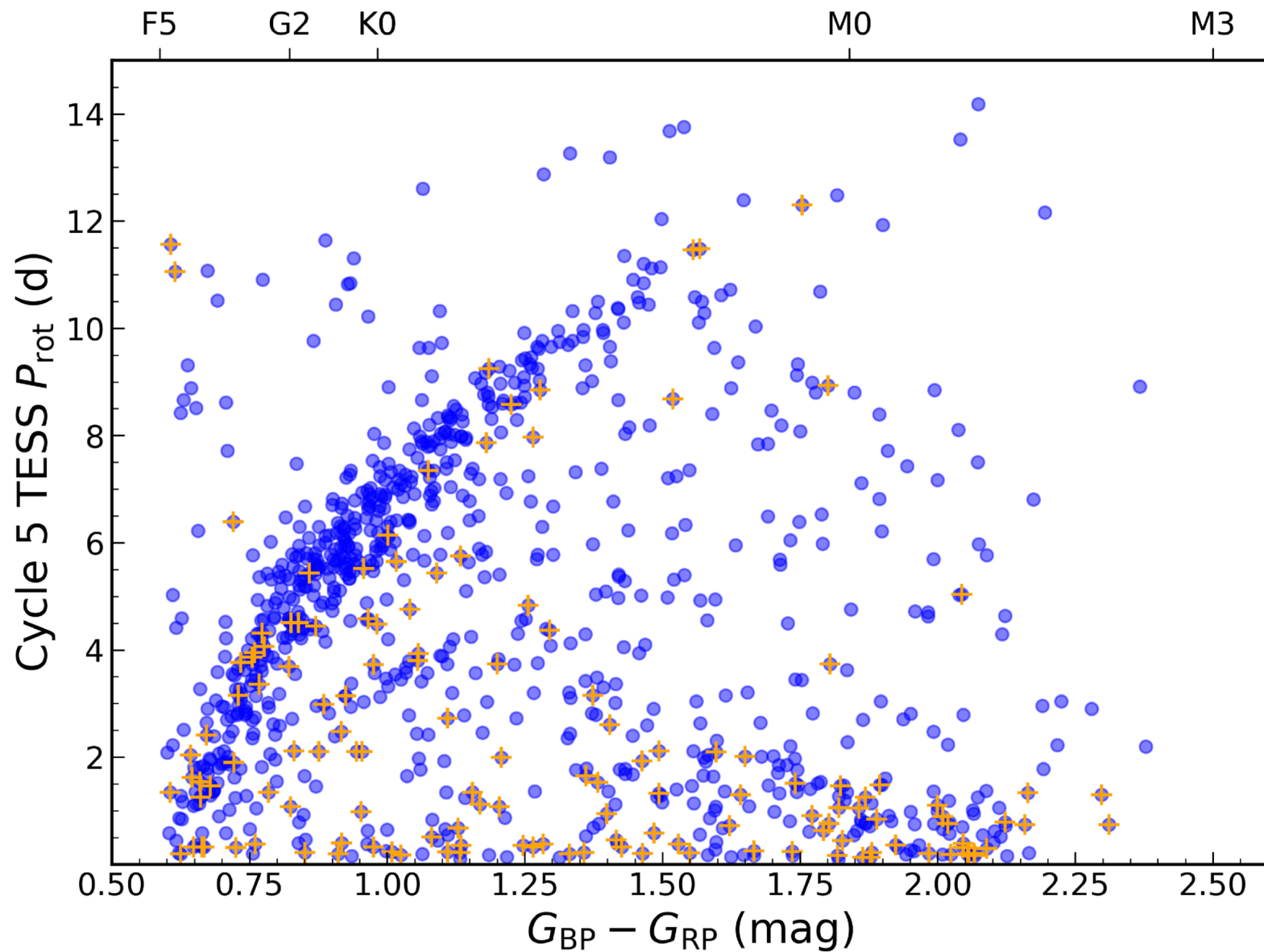
Figure 9. from Matthew S. Stafford et al 2026 Astron. J. 171 doi:10.3847/1538-3881/ae3c0c https://dx.doi.org/10.3847/1538-3881/ae3c0c © 2026. The Author(s). Published by the American Astronomical Society.
