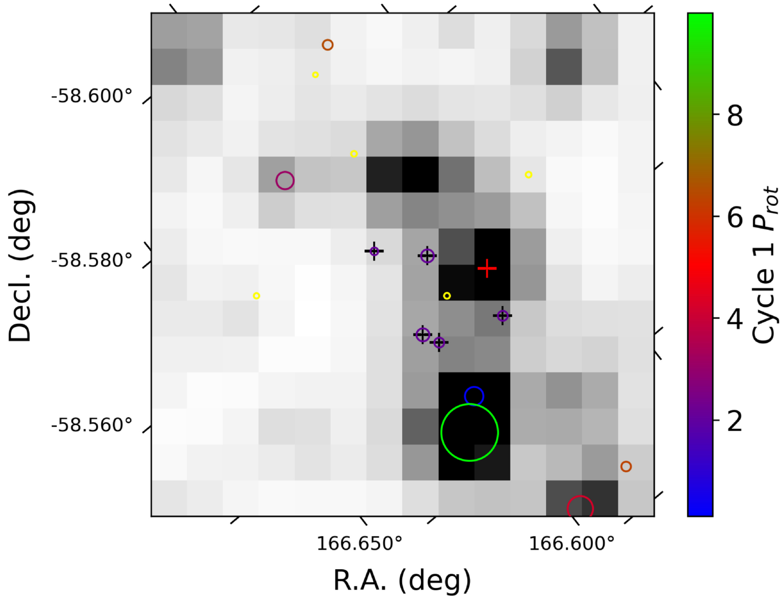
Figure 6. from Matthew S. Stafford et al 2026 Astron. J. 171 doi:10.3847/1538-3881/ae3c0c https://dx.doi.org/10.3847/1538-3881/ae3c0c © 2026. The Author(s). Published by the American Astronomical Society.
