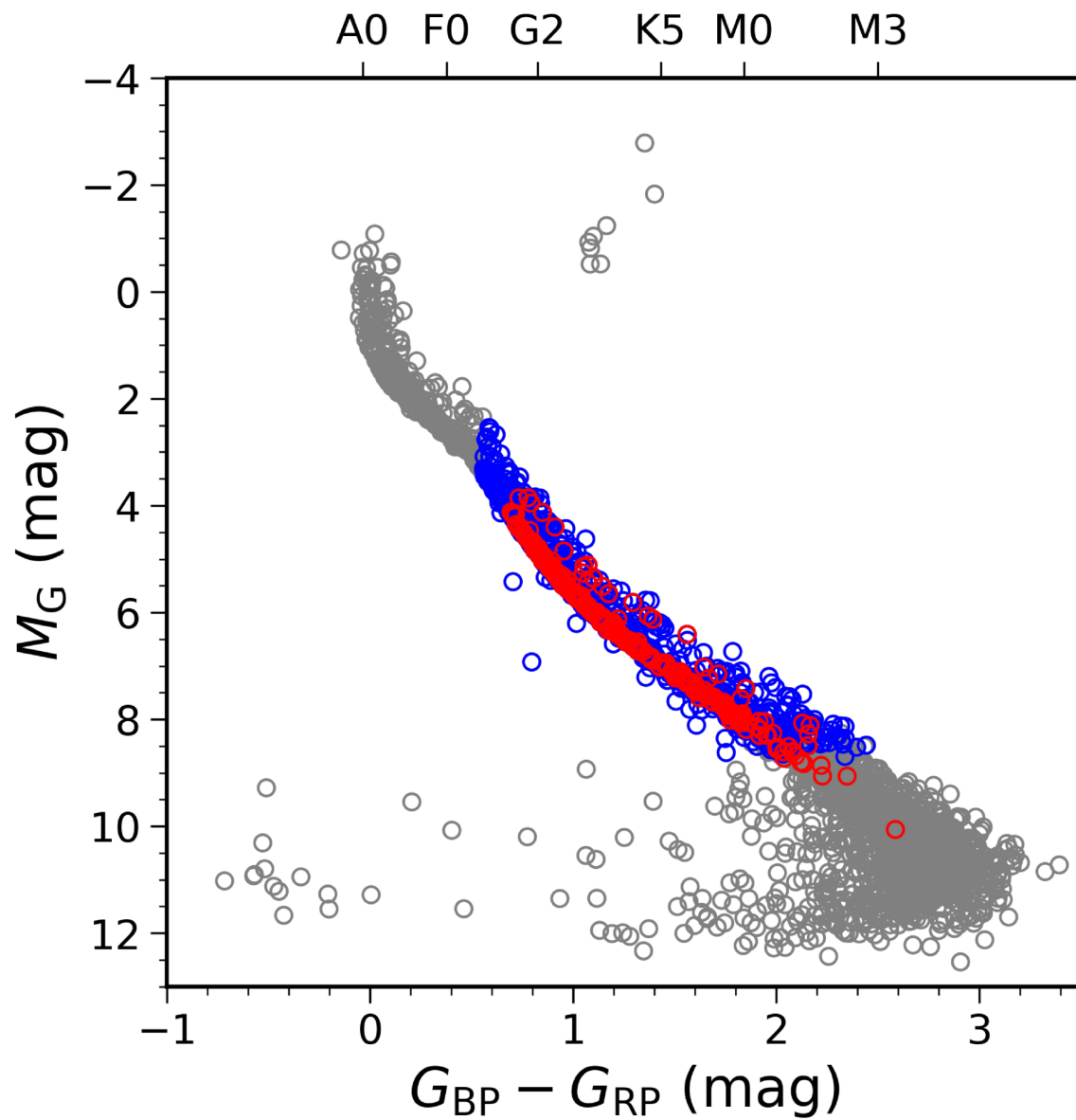
Figure 2. from Matthew S. Stafford et al 2026 Astron. J. 171 doi:10.3847/1538-3881/ae3c0c https://dx.doi.org/10.3847/1538-3881/ae3c0c © 2026. The Author(s). Published by the American Astronomical Society.
