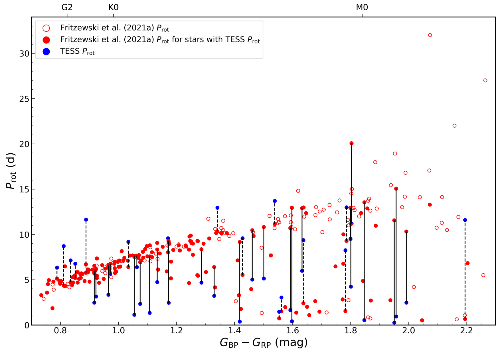
Figure 15. from Matthew S. Stafford et al 2026 Astron. J. 171 doi:10.3847/1538-3881/ae3c0c https://dx.doi.org/10.3847/1538-3881/ae3c0c © 2026. The Author(s). Published by the American Astronomical Society.
