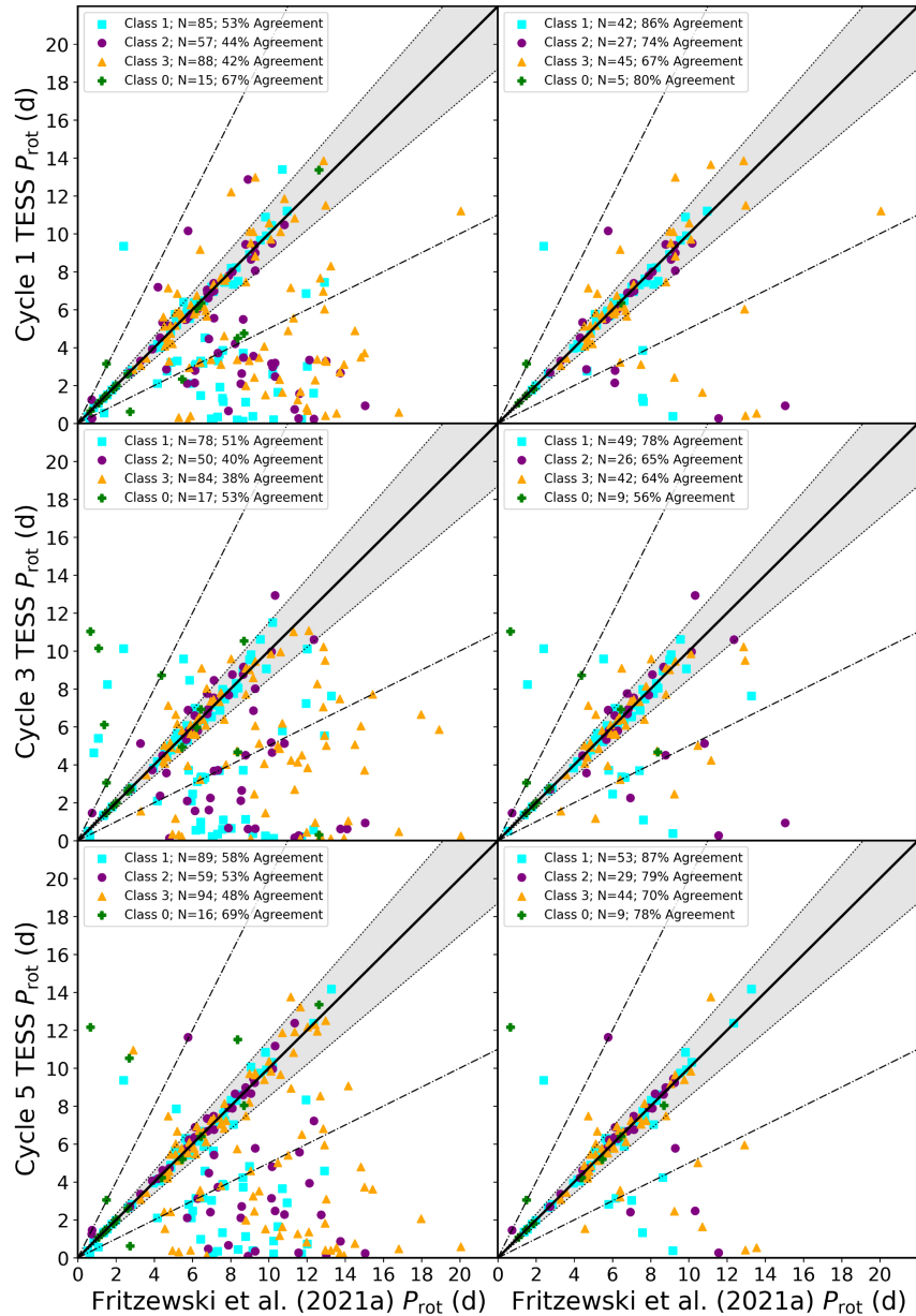
Figure 12. from Matthew S. Stafford et al 2026 Astron. J. 171 doi:10.3847/1538-3881/ae3c0c https://dx.doi.org/10.3847/1538-3881/ae3c0c © 2026. The Author(s). Published by the American Astronomical Society.
