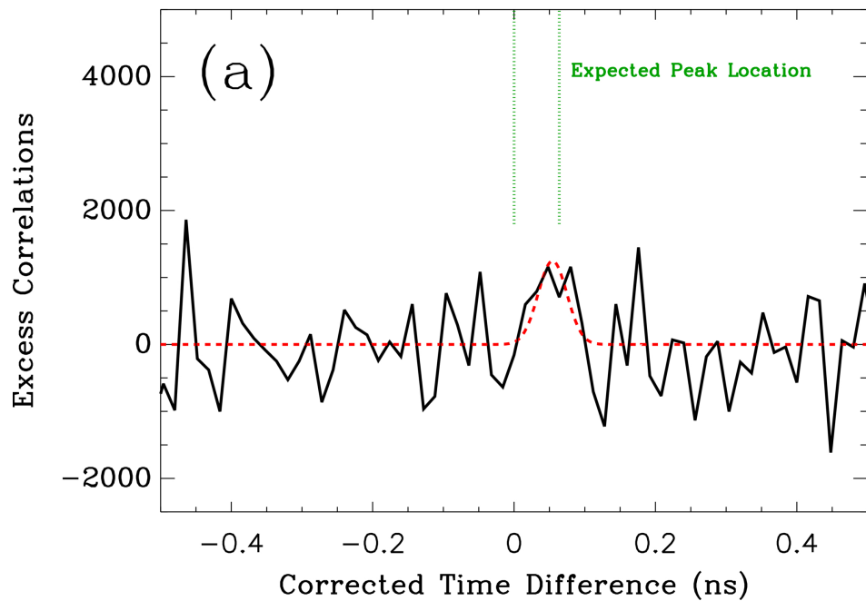
Figure 8. from Elliott P. Horch et al 2026 Astron. J. 171 doi:10.3847/1538-3881/ae3bd5 https://dx.doi.org/10.3847/1538-3881/ae3bd5 © 2026. The Author(s). Published by the American Astronomical Society.
