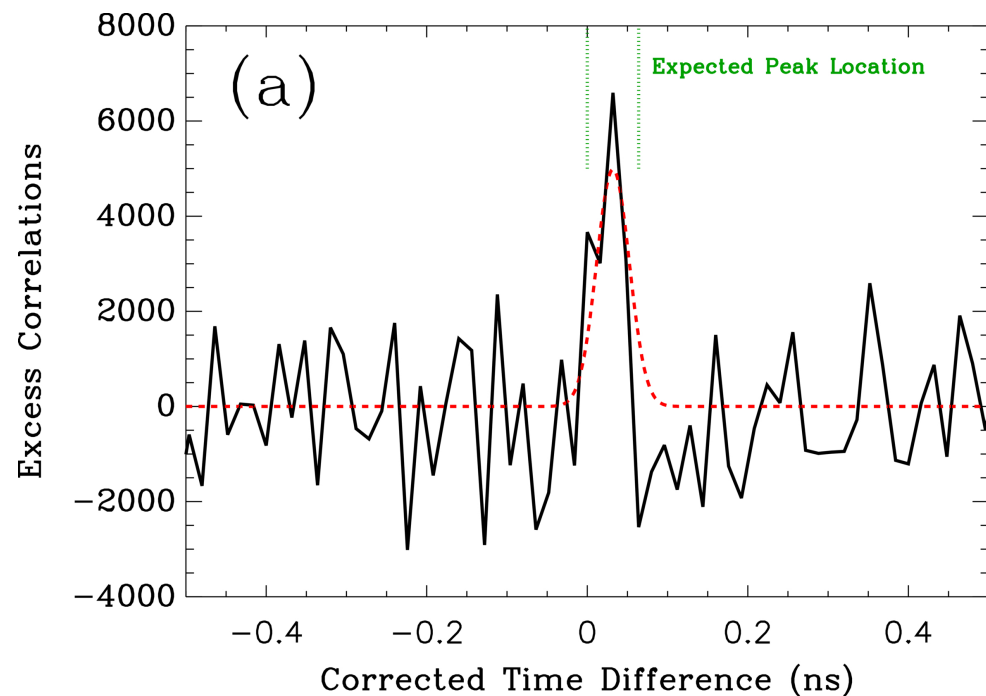
Figure 5. from Elliott P. Horch et al 2026 Astron. J. 171 doi:10.3847/1538-3881/ae3bd5 https://dx.doi.org/10.3847/1538-3881/ae3bd5 © 2026. The Author(s). Published by the American Astronomical Society.
