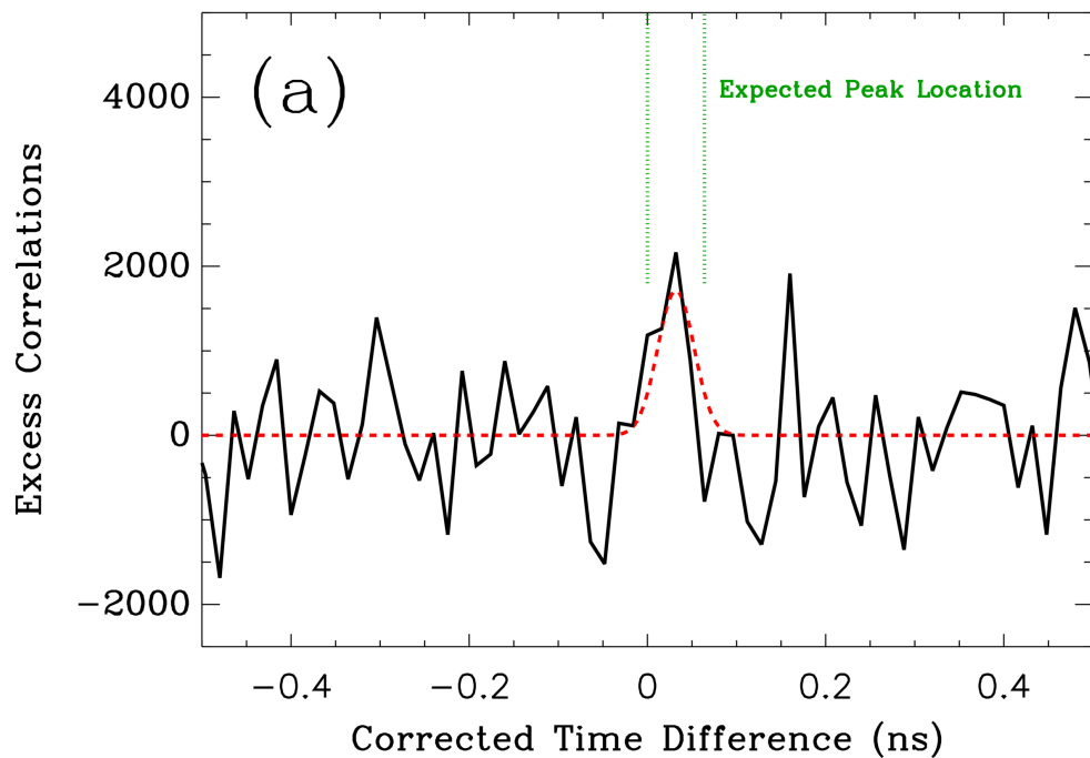
Figure 4. from Elliott P. Horch et al 2026 Astron. J. 171 doi:10.3847/1538-3881/ae3bd5 https://dx.doi.org/10.3847/1538-3881/ae3bd5 © 2026. The Author(s). Published by the American Astronomical Society.
