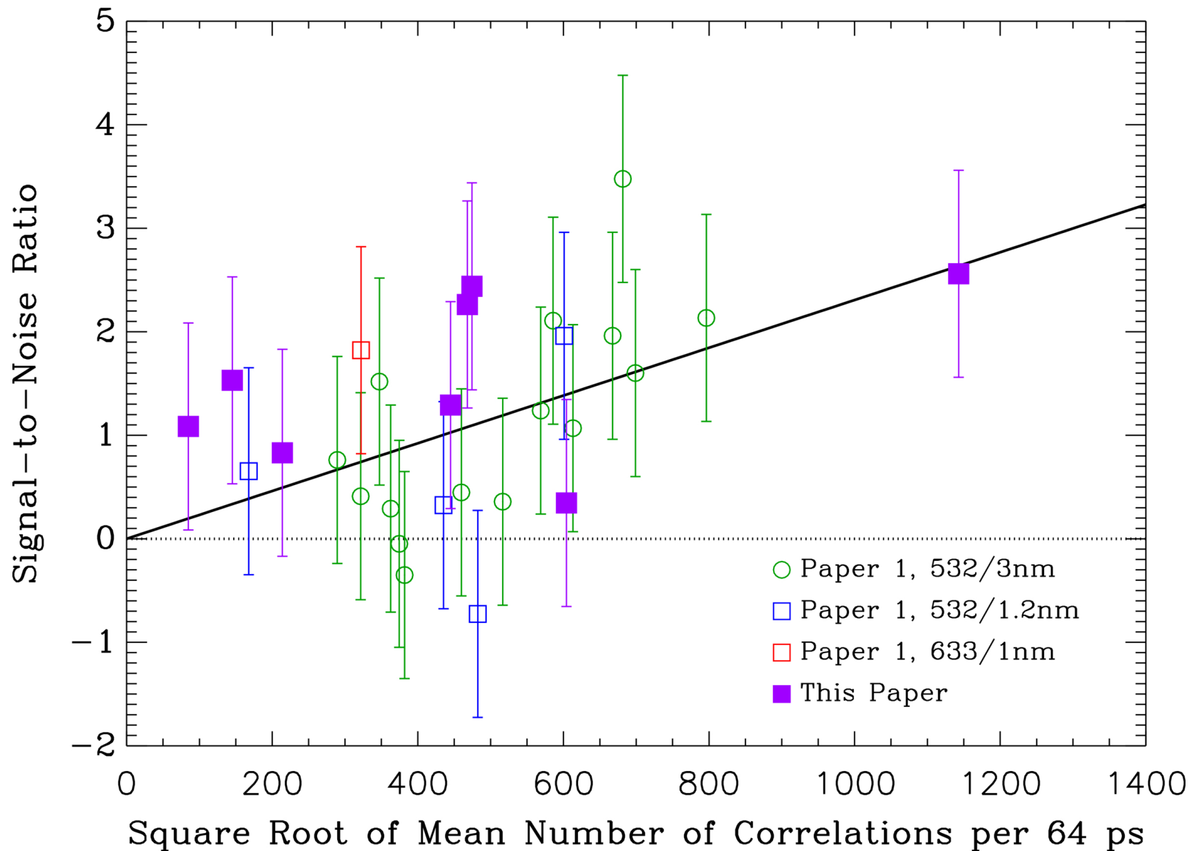
Figure 3. from Elliott P. Horch et al 2026 Astron. J. 171 doi:10.3847/1538-3881/ae3bd5 https://dx.doi.org/10.3847/1538-3881/ae3bd5 © 2026. The Author(s). Published by the American Astronomical Society.
