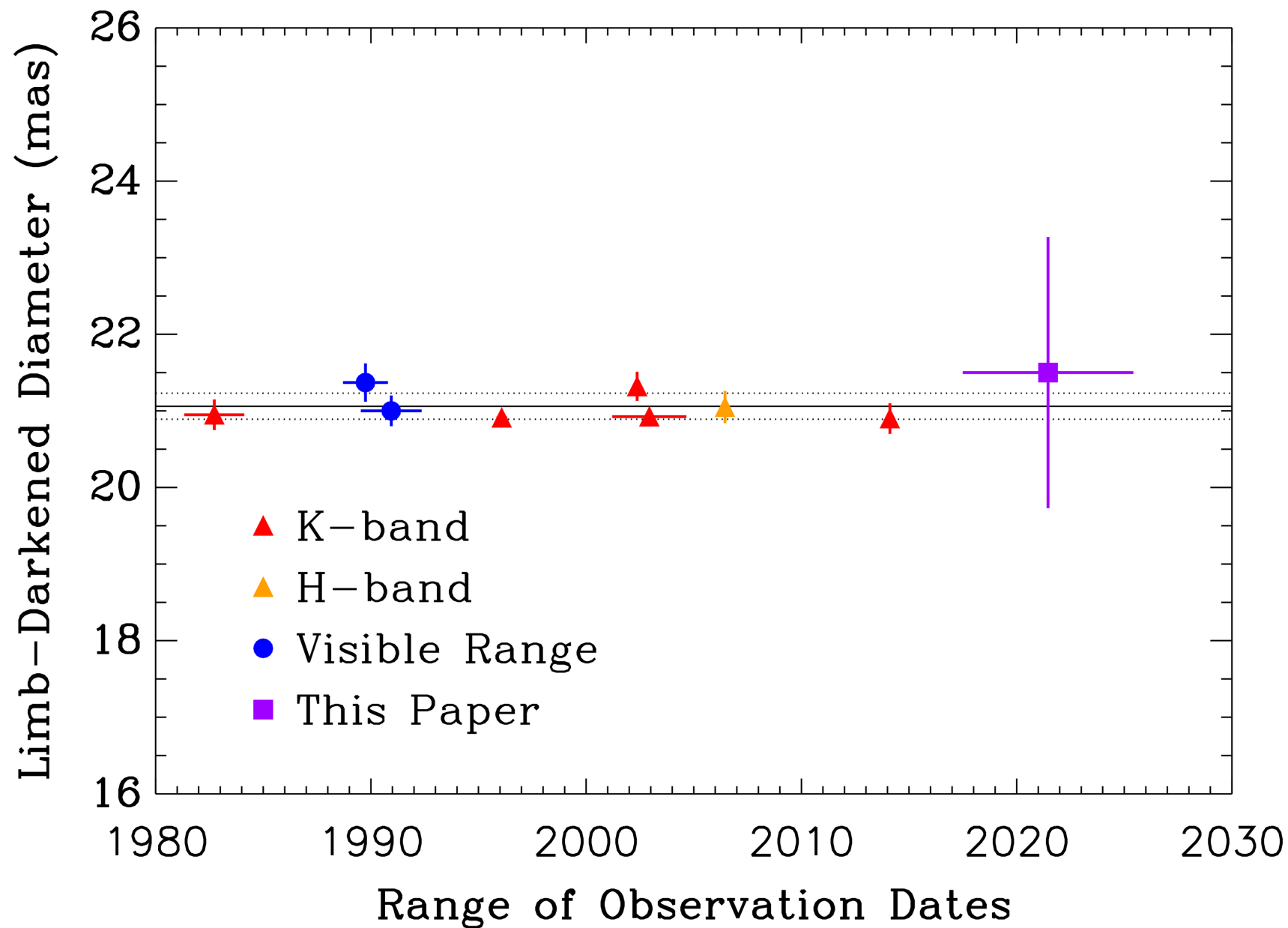
Figure 12. from Elliott P. Horch et al 2026 Astron. J. 171 doi:10.3847/1538-3881/ae3bd5 https://dx.doi.org/10.3847/1538-3881/ae3bd5 © 2026. The Author(s). Published by the American Astronomical Society.
