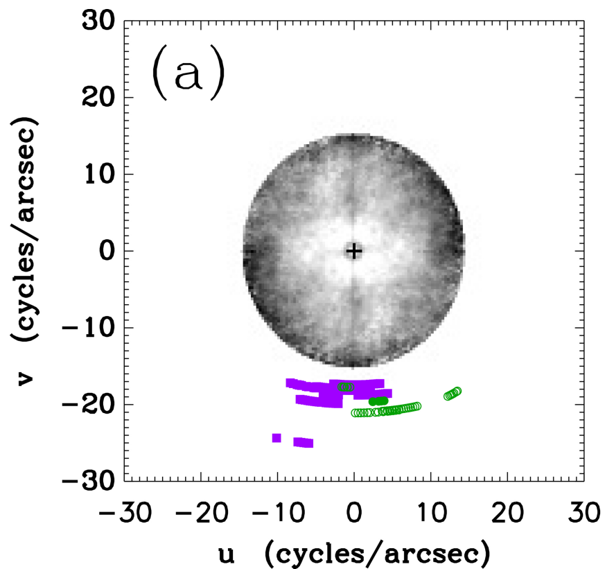
Figure 11. from Elliott P. Horch et al 2026 Astron. J. 171 doi:10.3847/1538-3881/ae3bd5 https://dx.doi.org/10.3847/1538-3881/ae3bd5 © 2026. The Author(s). Published by the American Astronomical Society.
