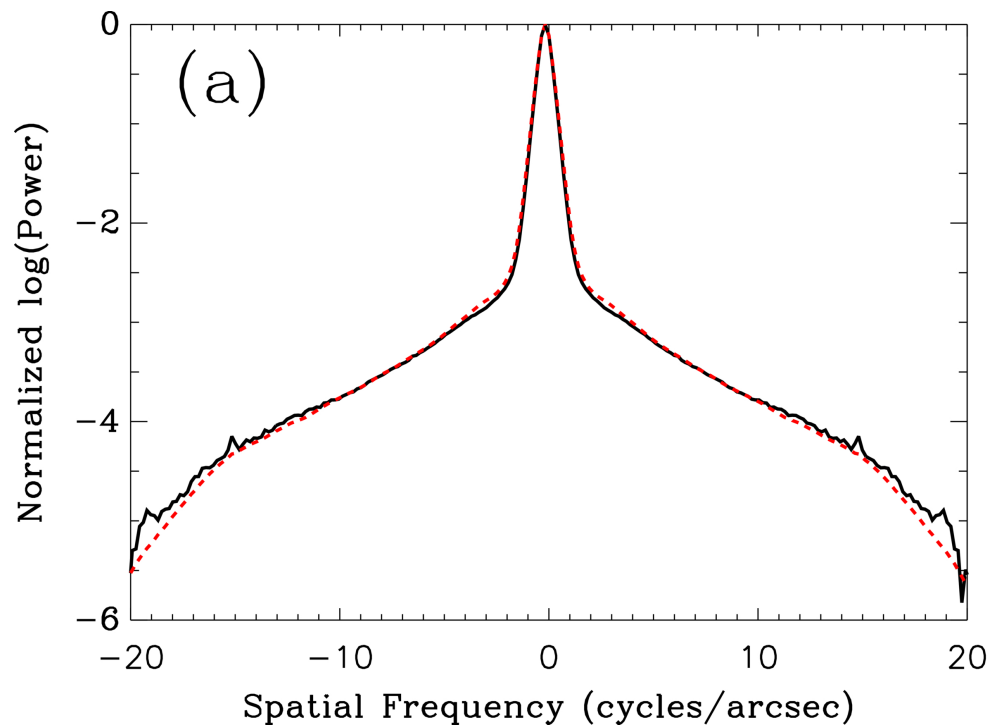
Figure 10. from Elliott P. Horch et al 2026 Astron. J. 171 doi:10.3847/1538-3881/ae3bd5 https://dx.doi.org/10.3847/1538-3881/ae3bd5 © 2026. The Author(s). Published by the American Astronomical Society.
