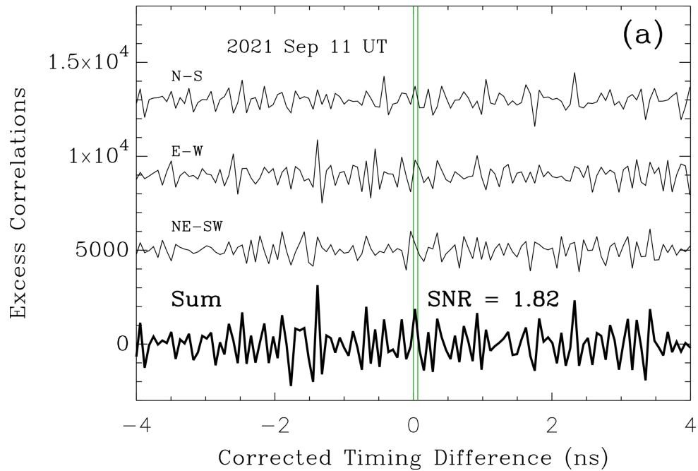
Figure 1. from Elliott P. Horch et al 2026 Astron. J. 171 doi:10.3847/1538-3881/ae3bd5 https://dx.doi.org/10.3847/1538-3881/ae3bd5 © 2026. The Author(s). Published by the American Astronomical Society.
