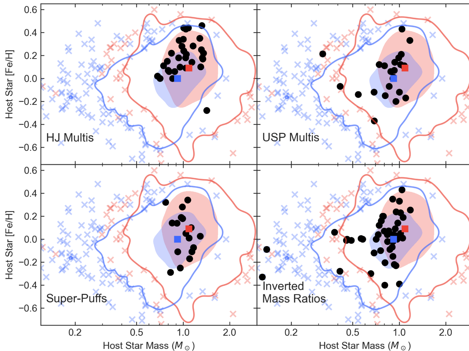
Figure 6. from Alex R. Howe et al 2026 Astron. J. 171 doi:10.3847/1538-3881/ae3aa6 https://dx.doi.org/10.3847/1538-3881/ae3aa6 © 2026. The Author(s). Published by the American Astronomical Society.
