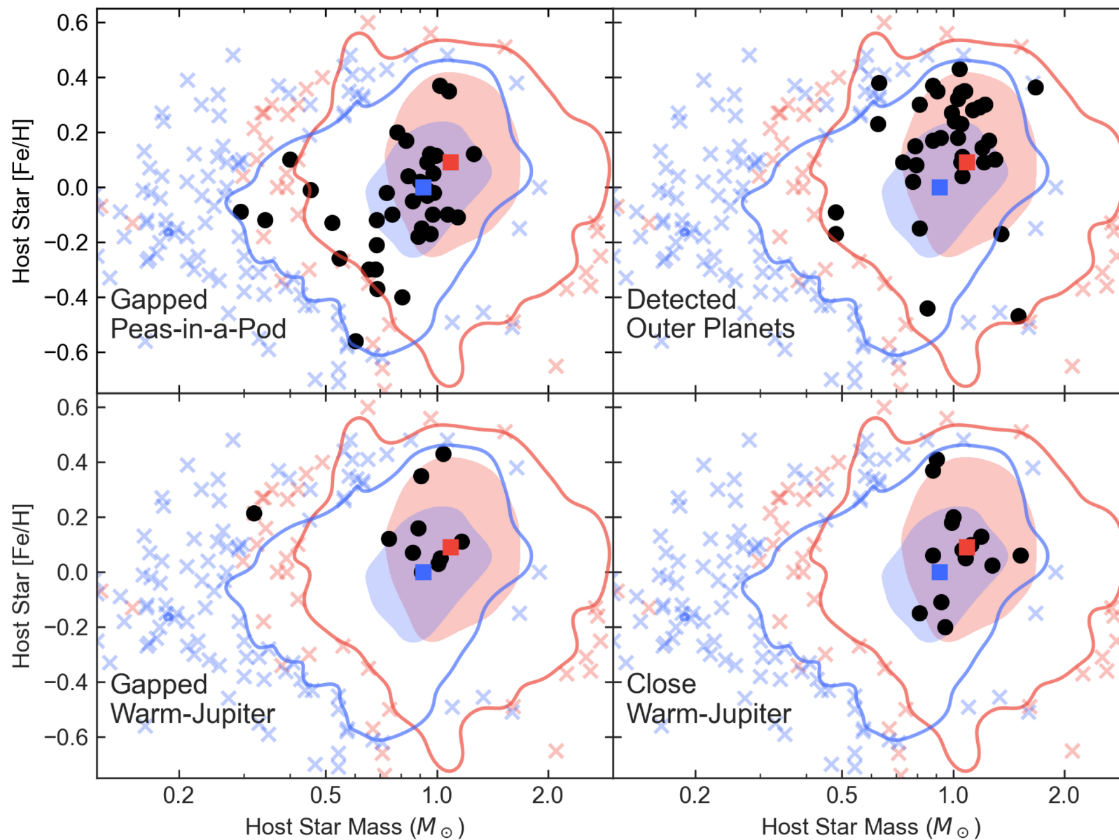
Figure 5. from Alex R. Howe et al 2026 Astron. J. 171 doi:10.3847/1538-3881/ae3aa6 https://dx.doi.org/10.3847/1538-3881/ae3aa6 © 2026. The Author(s). Published by the American Astronomical Society.
