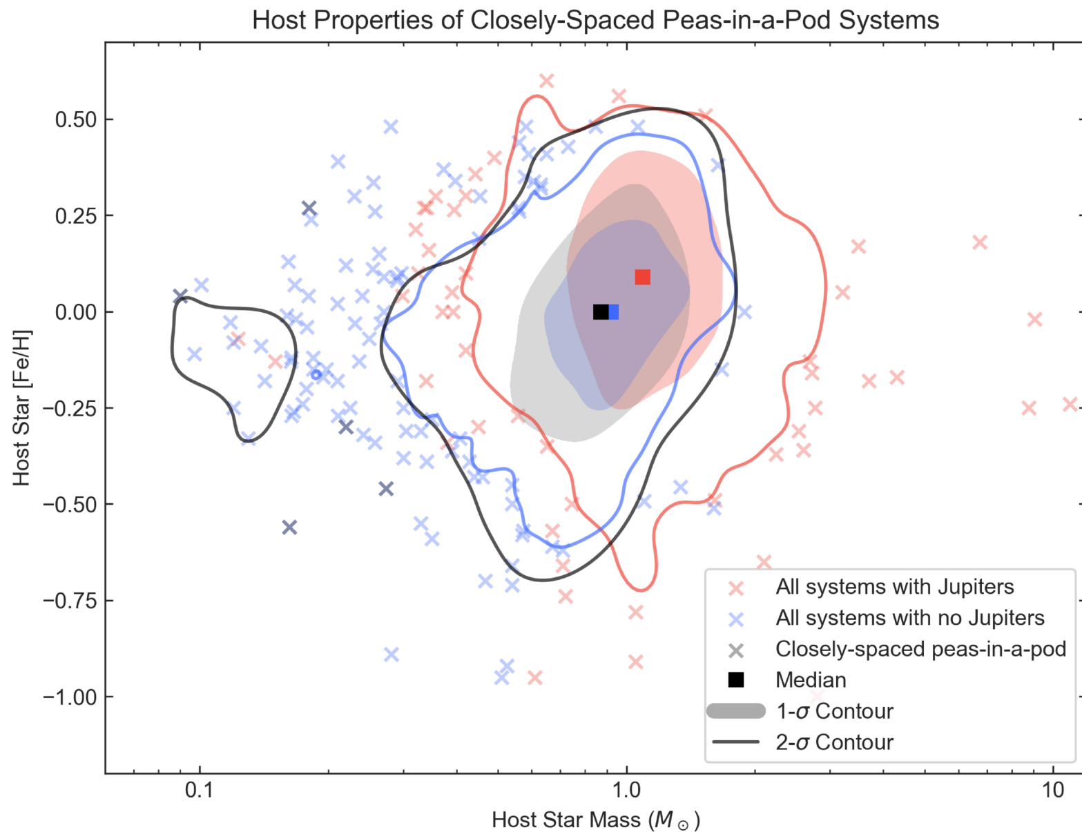
Figure 4. from Alex R. Howe et al 2026 Astron. J. 171 doi:10.3847/1538-3881/ae3aa6 https://dx.doi.org/10.3847/1538-3881/ae3aa6 © 2026. The Author(s). Published by the American Astronomical Society.
