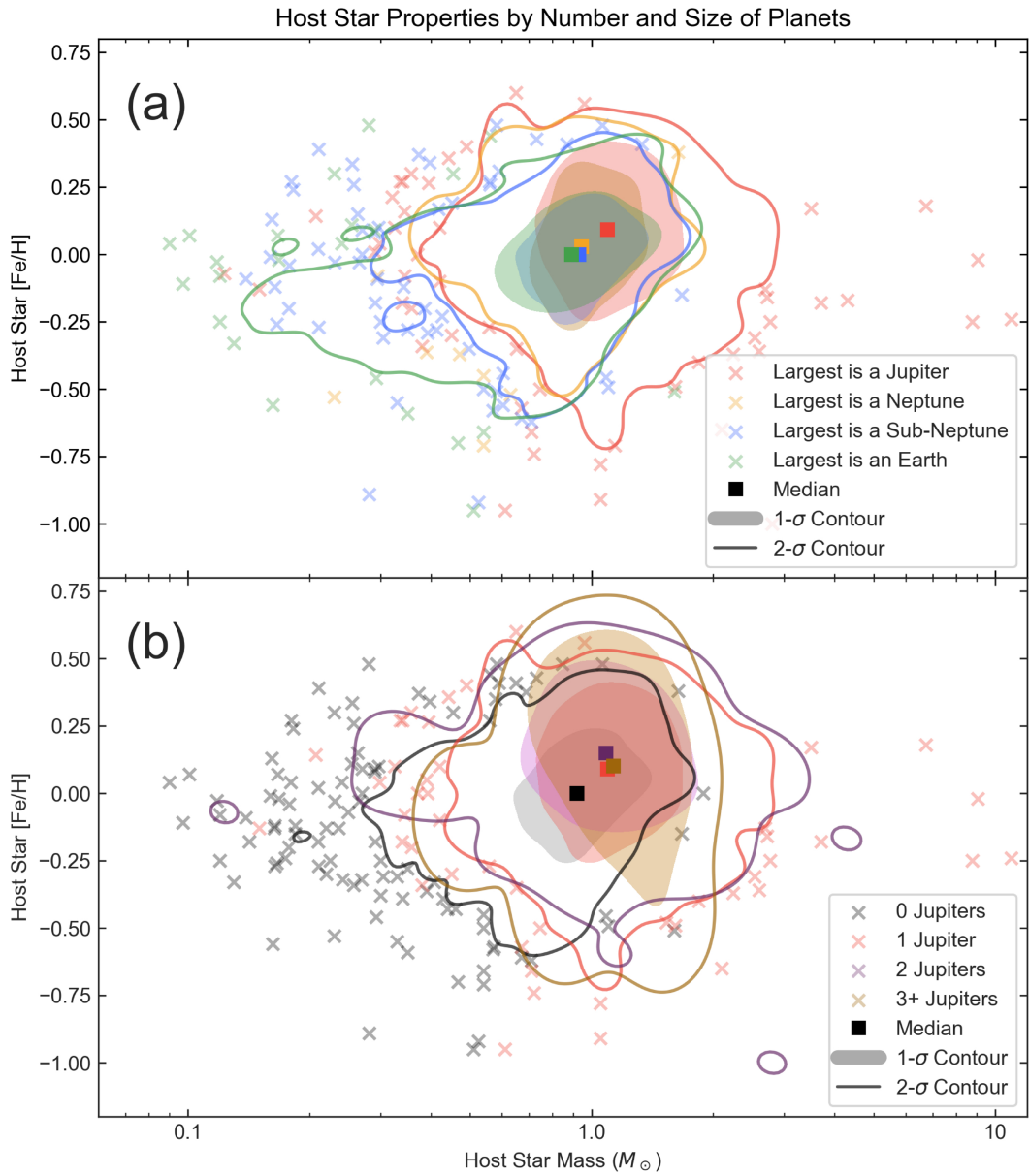
Figure 3. from Alex R. Howe et al 2026 Astron. J. 171 doi:10.3847/1538-3881/ae3aa6 https://dx.doi.org/10.3847/1538-3881/ae3aa6 © 2026. The Author(s). Published by the American Astronomical Society.
