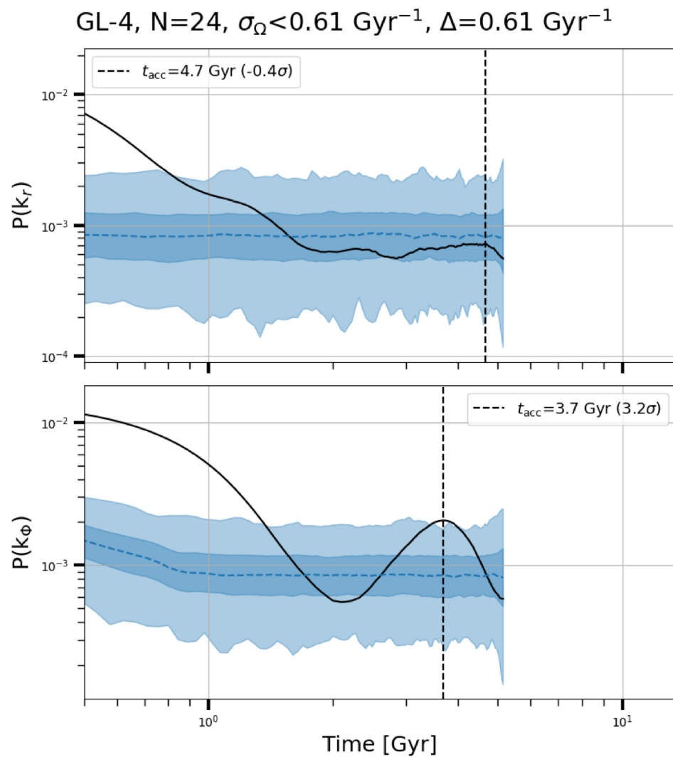
Figure 8. from Hefan Li et al 2026 Astron. J. 171 doi:10.3847/1538-3881/ae3a83 https://dx.doi.org/10.3847/1538-3881/ae3a83 © 2026. The Author(s). Published by the American Astronomical Society.
