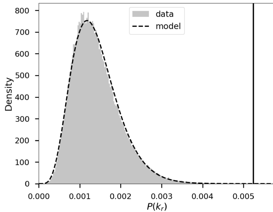
Figure 6. from Hefan Li et al 2026 Astron. J. 171 doi:10.3847/1538-3881/ae3a83 https://dx.doi.org/10.3847/1538-3881/ae3a83 © 2026. The Author(s). Published by the American Astronomical Society.
